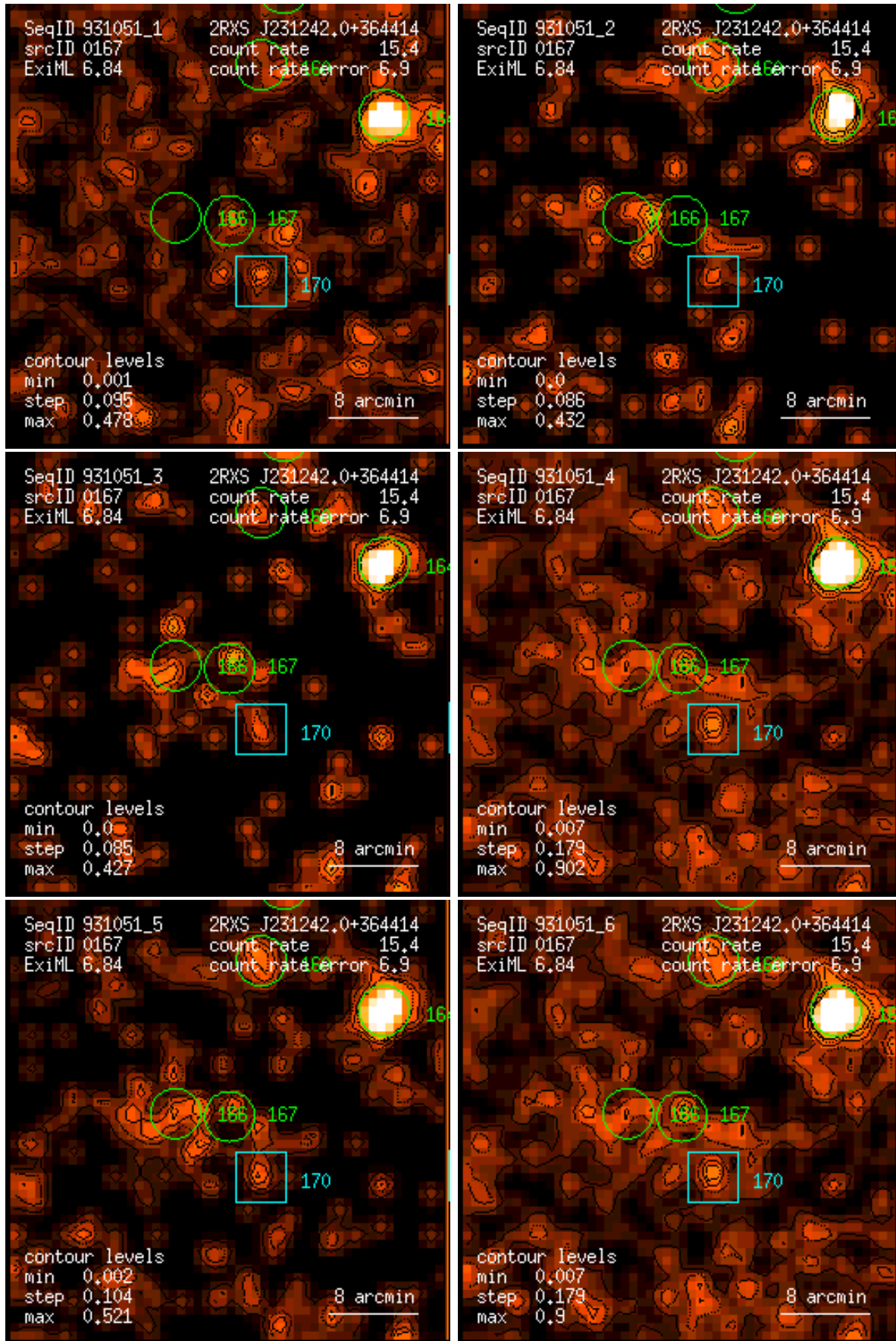
Figure 167: RASS 931051: detection 0167: band rate images, Gaussian filter: (1) PSPC channels 11 – 41, (2) 52 – 90, (3) 91 – 201, (4) 11 – 235, (5) 52 – 201, (6) 11 – 201. Broad band rates in counts/ks. Band rate contour levels in counts/ks/arcmin 2 .
