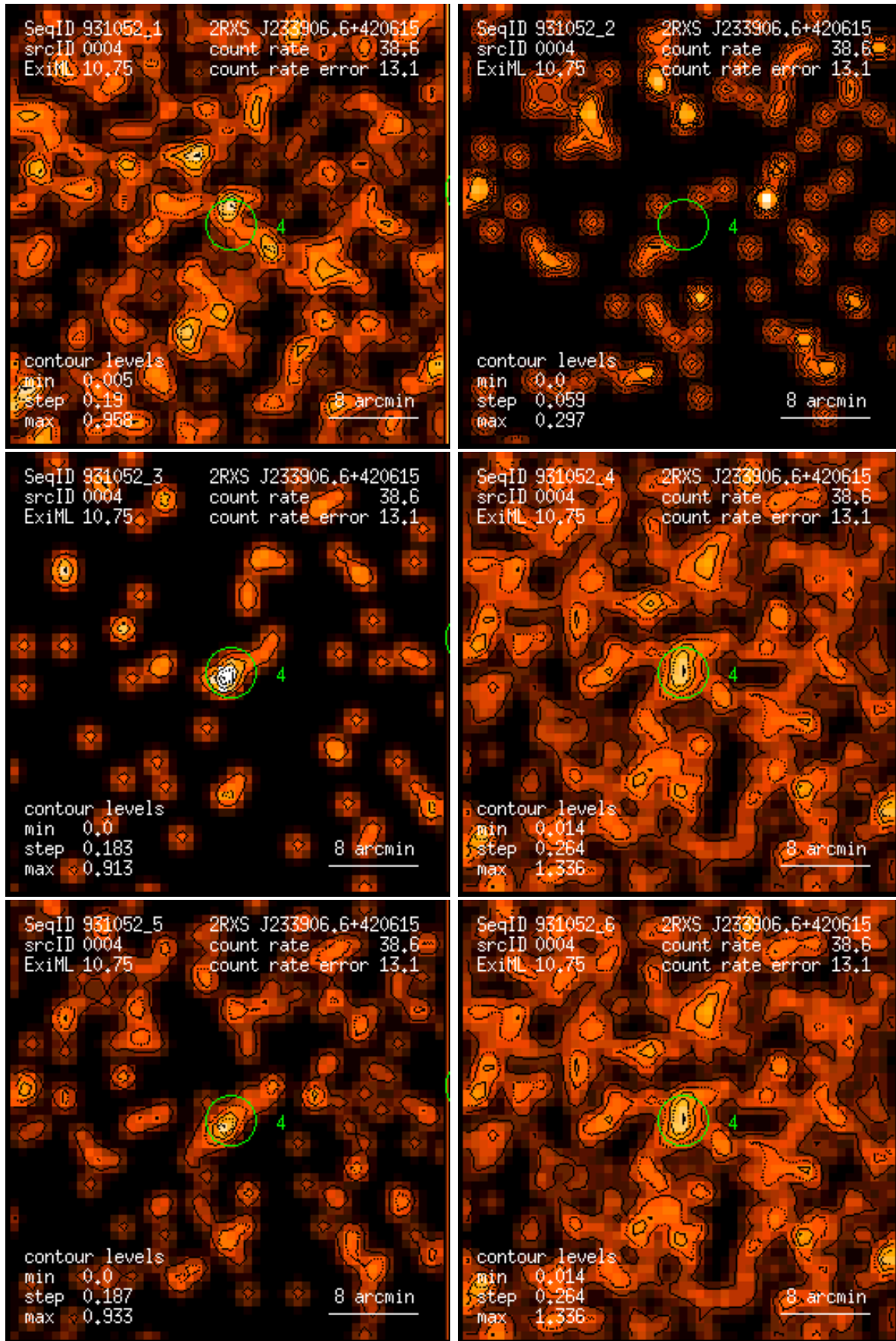
Figure 4: RASS 931052: detection 0004: band rate images, Gaussian filter: (1) PSPC channels 11 – 41, (2) 52 – 90, (3) 91 – 201, (4) 11 – 235, (5) 52 – 201, (6) 11 – 201. Broad band rates in counts/ks. Band rate contour levels in counts/ks/arcmin 2 .
