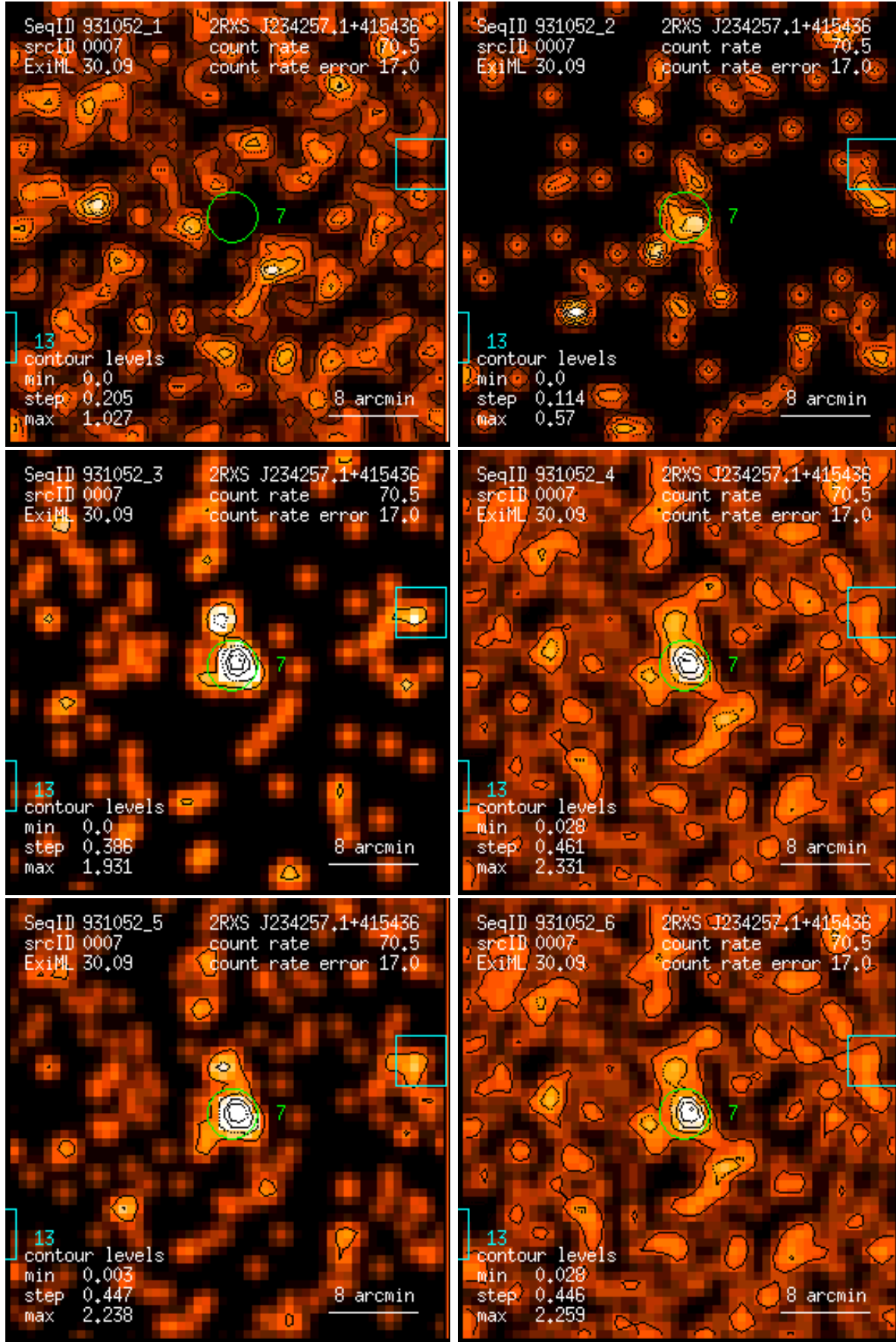
Figure 7: RASS 931052: detection 0007: band rate images, Gaussian filter: (1) PSPC channels 11 – 41, (2) 52 – 90, (3) 91 – 201, (4) 11 – 235, (5) 52 – 201, (6) 11 – 201. Broad band rates in counts/ks. Band rate contour levels in counts/ks/arcmin 2 .
