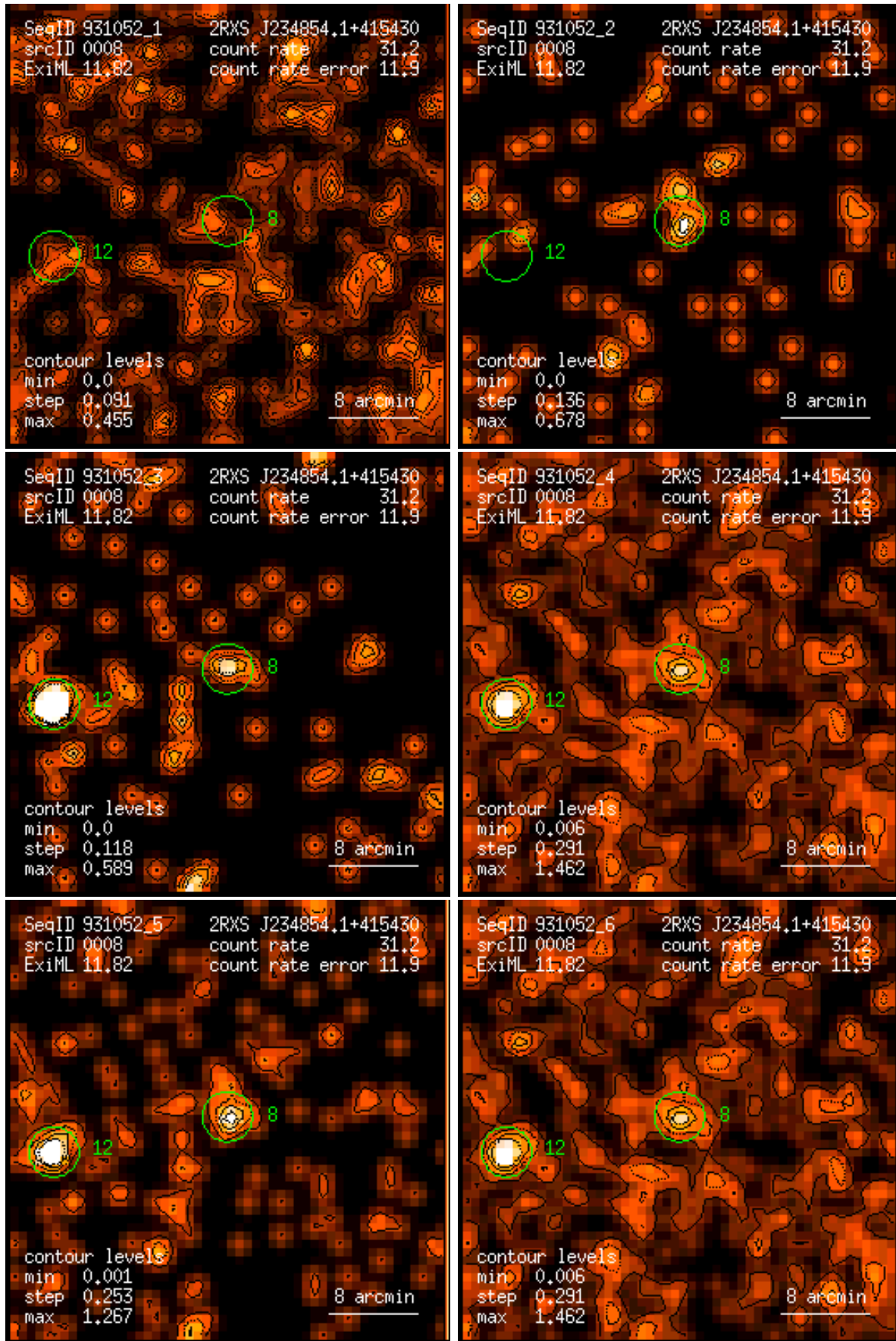
Figure 8: RASS 931052: detection 0008: band rate images, Gaussian filter: (1) PSPC channels 11 – 41, (2) 52 – 90, (3) 91 – 201, (4) 11 – 235, (5) 52 – 201, (6) 11 – 201. Broad band rates in counts/ks. Band rate contour levels in counts/ks/arcmin 2 .
