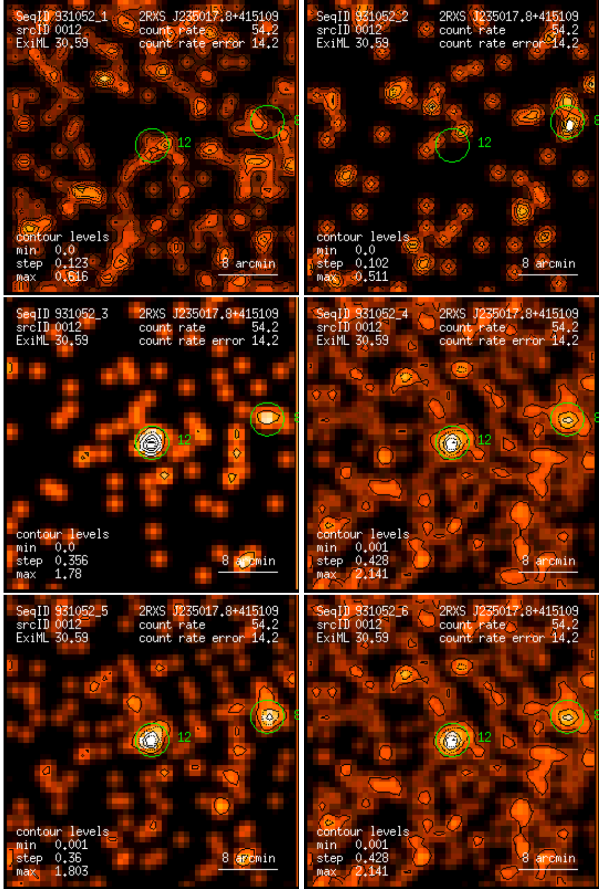
Figure 12: RASS 931052: detection 0012: band rate images, Gaussian filter: (1) PSPC channels 11 – 41, (2) 52 – 90, (3) 91 – 201, (4) 11 – 235, (5) 52 – 201, (6) 11 – 201. Broad band rates in counts/ks. Band rate contour levels in counts/ks/arcmin 2 .
