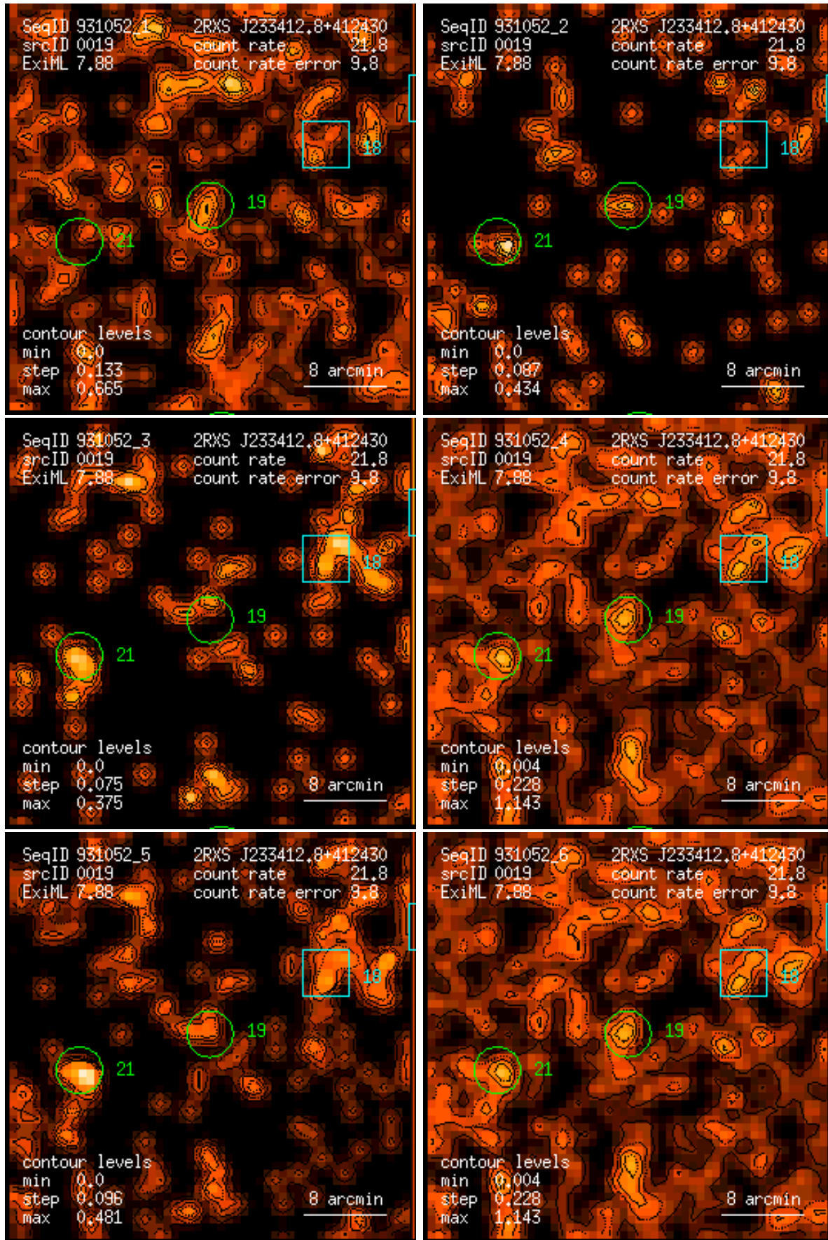
Figure 19: RASS 931052: detection 0019: band rate images, Gaussian filter: (1) PSPC channels 11 – 41, (2) 52 – 90, (3) 91 – 201, (4) 11 – 235, (5) 52 – 201, (6) 11 – 201. Broad band rates in counts/ks. Band rate contour levels in counts/ks/arcmin 2 .
