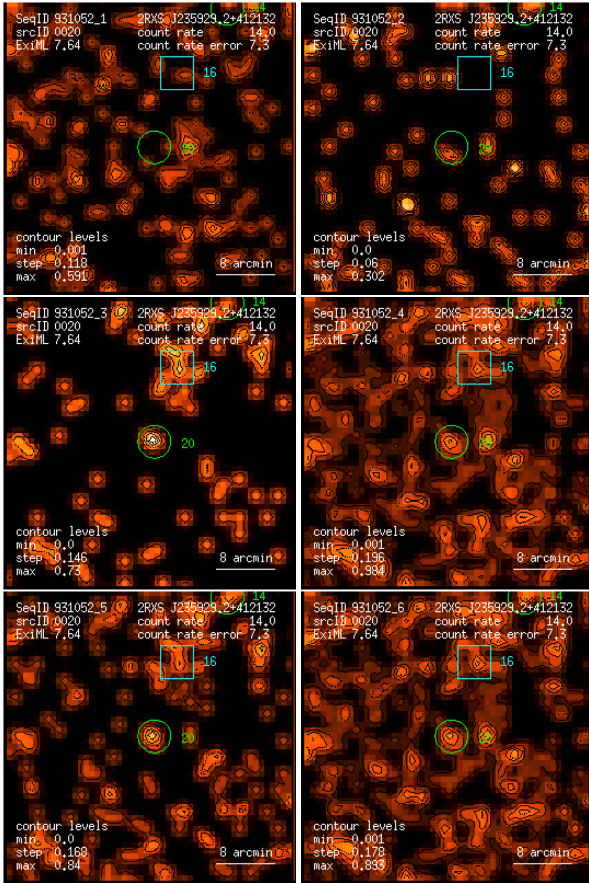
Figure 20: RASS 931052: detection 0020: band rate images, Gaussian filter: (1) PSPC channels 11 – 41, (2) 52 – 90, (3) 91 – 201, (4) 11 – 235, (5) 52 – 201, (6) 11 – 201. Broad band rates in counts/ks. Band rate contour levels in counts/ks/arcmin 2 .
