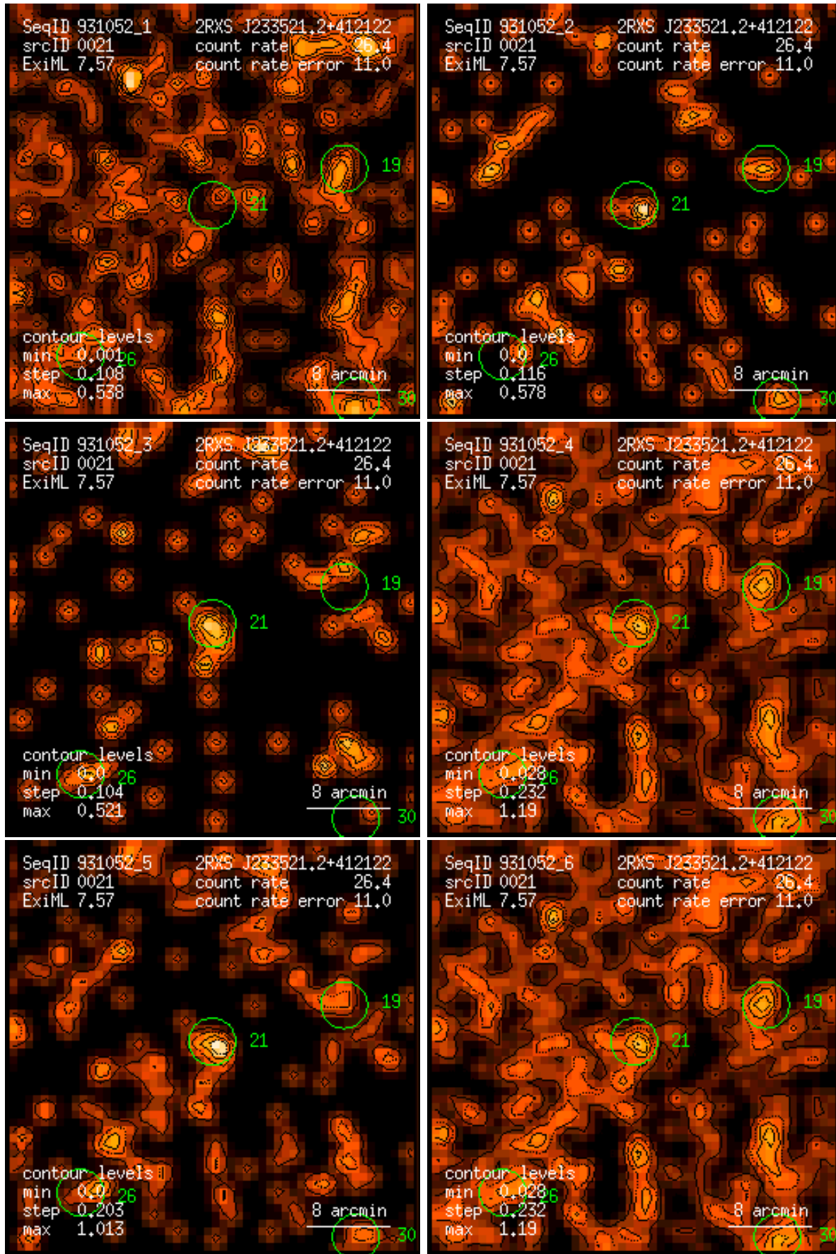
Figure 21: RASS 931052: detection 0021: band rate images, Gaussian filter: (1) PSPC channels 11 – 41, (2) 52 – 90, (3) 91 – 201, (4) 11 – 235, (5) 52 – 201, (6) 11 – 201. Broad band rates in counts/ks. Band rate contour levels in counts/ks/arcmin 2 .
