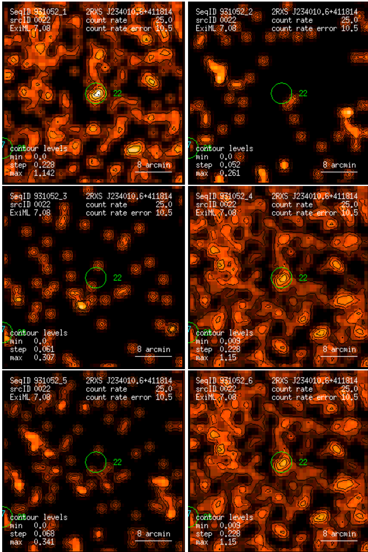
Figure 22: RASS 931052: detection 0022: band rate images, Gaussian filter: (1) PSPC channels 11 – 41, (2) 52 – 90, (3) 91 – 201, (4) 11 – 235, (5) 52 – 201, (6) 11 – 201. Broad band rates in counts/ks. Band rate contour levels in counts/ks/arcmin 2 .
