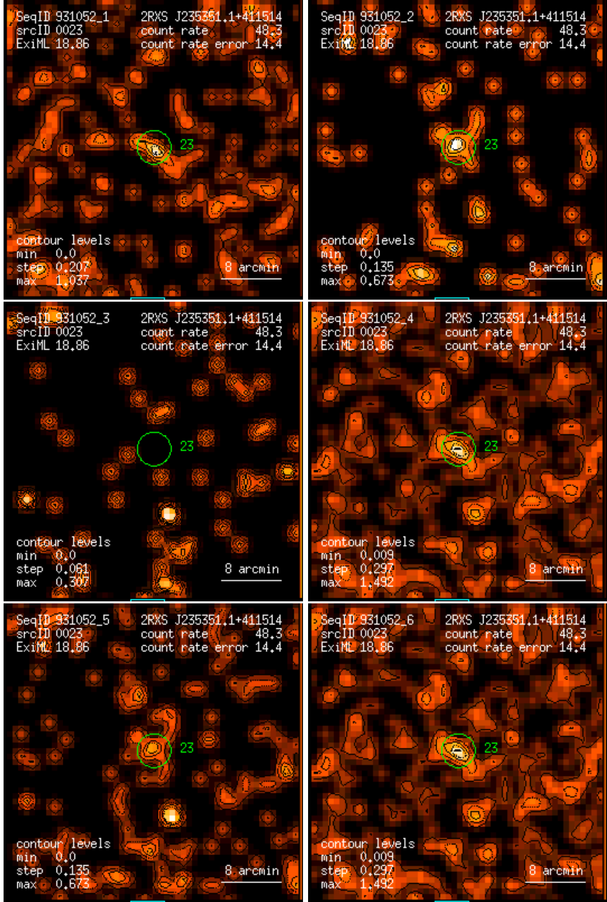
Figure 23: RASS 931052: detection 0023: band rate images, Gaussian filter: (1) PSPC channels 11 – 41, (2) 52 – 90, (3) 91 – 201, (4) 11 – 235, (5) 52 – 201, (6) 11 – 201. Broad band rates in counts/ks. Band rate contour levels in counts/ks/arcmin 2 .
