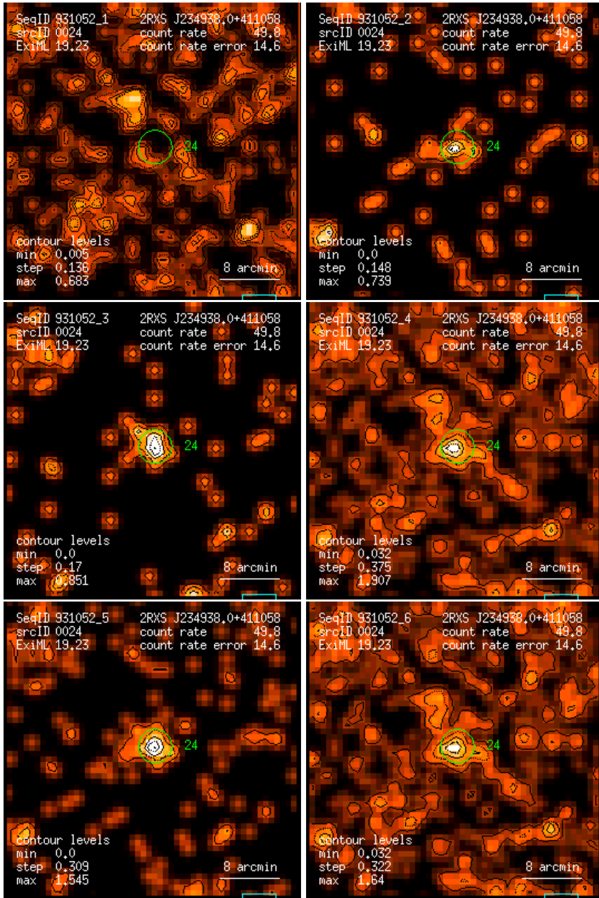
Figure 24: RASS 931052: detection 0024: band rate images, Gaussian filter: (1) PSPC channels 11 – 41, (2) 52 – 90, (3) 91 – 201, (4) 11 – 235, (5) 52 – 201, (6) 11 – 201. Broad band rates in counts/ks. Band rate contour levels in counts/ks/arcmin 2 .
