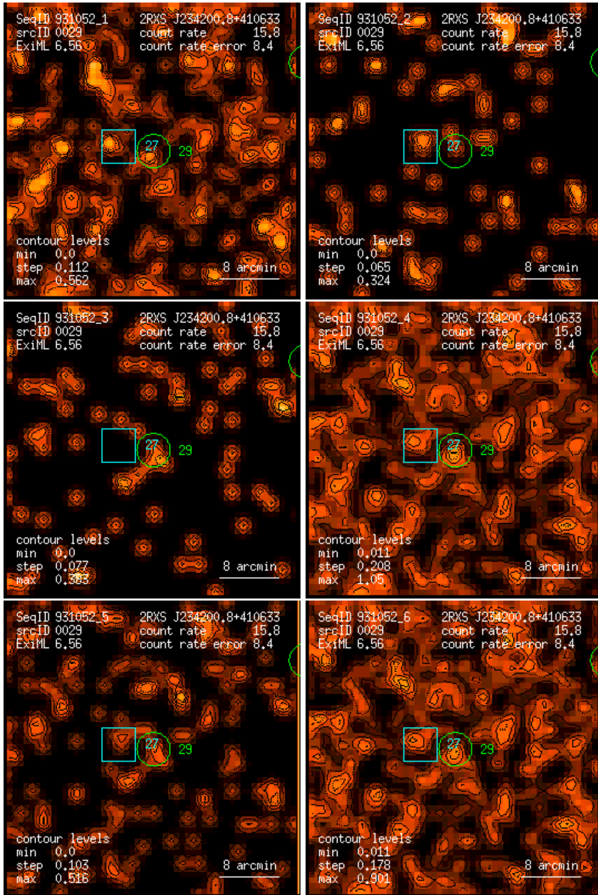
Figure 29: RASS 931052: detection 0029: band rate images, Gaussian filter: (1) PSPC channels 11 – 41, (2) 52 – 90, (3) 91 – 201, (4) 11 – 235, (5) 52 – 201, (6) 11 – 201. Broad band rates in counts/ks. Band rate contour levels in counts/ks/arcmin 2 .
