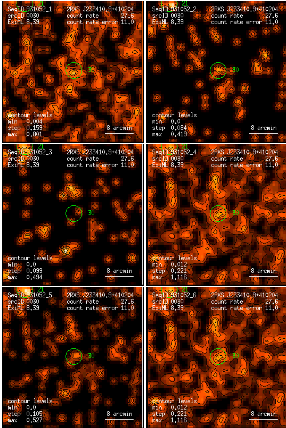
Figure 30: RASS 931052: detection 0030: band rate images, Gaussian filter: (1) PSPC channels 11 – 41, (2) 52 – 90, (3) 91 – 201, (4) 11 – 235, (5) 52 – 201, (6) 11 – 201. Broad band rates in counts/ks. Band rate contour levels in counts/ks/arcmin 2 .
