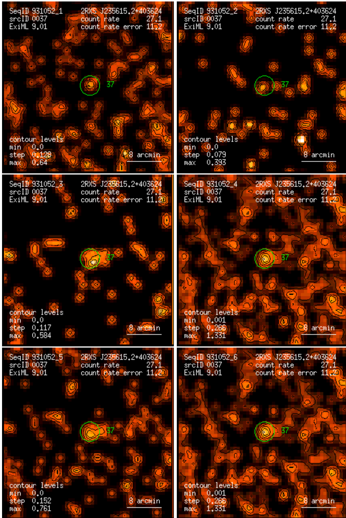
Figure 37: RASS 931052: detection 0037: band rate images, Gaussian filter: (1) PSPC channels 11 – 41, (2) 52 – 90, (3) 91 – 201, (4) 11 – 235, (5) 52 – 201, (6) 11 – 201. Broad band rates in counts/ks. Band rate contour levels in counts/ks/arcmin 2 .
