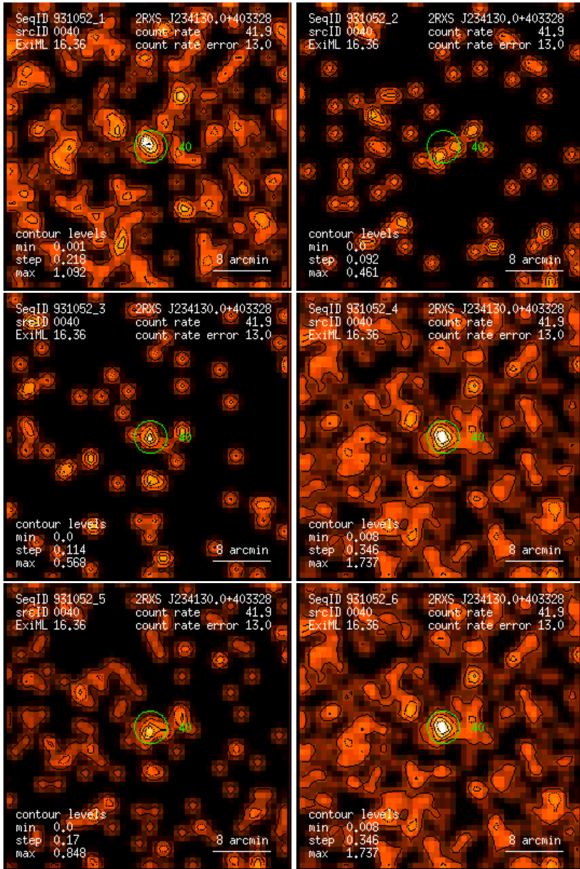
Figure 40: RASS 931052: detection 0040: band rate images, Gaussian filter: (1) PSPC channels 11 – 41, (2) 52 – 90, (3) 91 – 201, (4) 11 – 235, (5) 52 – 201, (6) 11 – 201. Broad band rates in counts/ks. Band rate contour levels in counts/ks/arcmin 2 .
