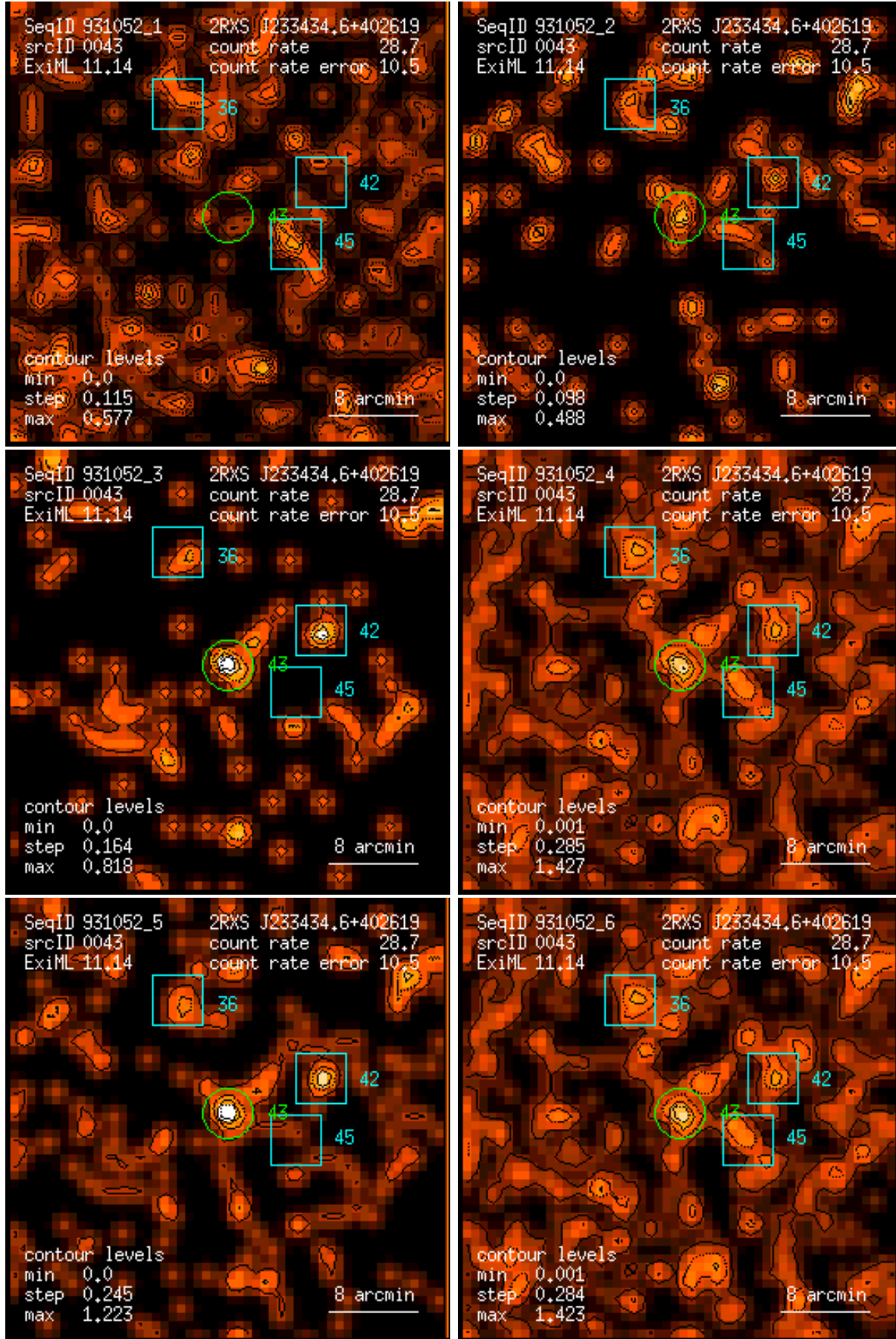
Figure 43: RASS 931052: detection 0043: band rate images, Gaussian filter: (1) PSPC channels 11 – 41, (2) 52 – 90, (3) 91 – 201, (4) 11 – 235, (5) 52 – 201, (6) 11 – 201. Broad band rates in counts/ks. Band rate contour levels in counts/ks/arcmin 2 .
