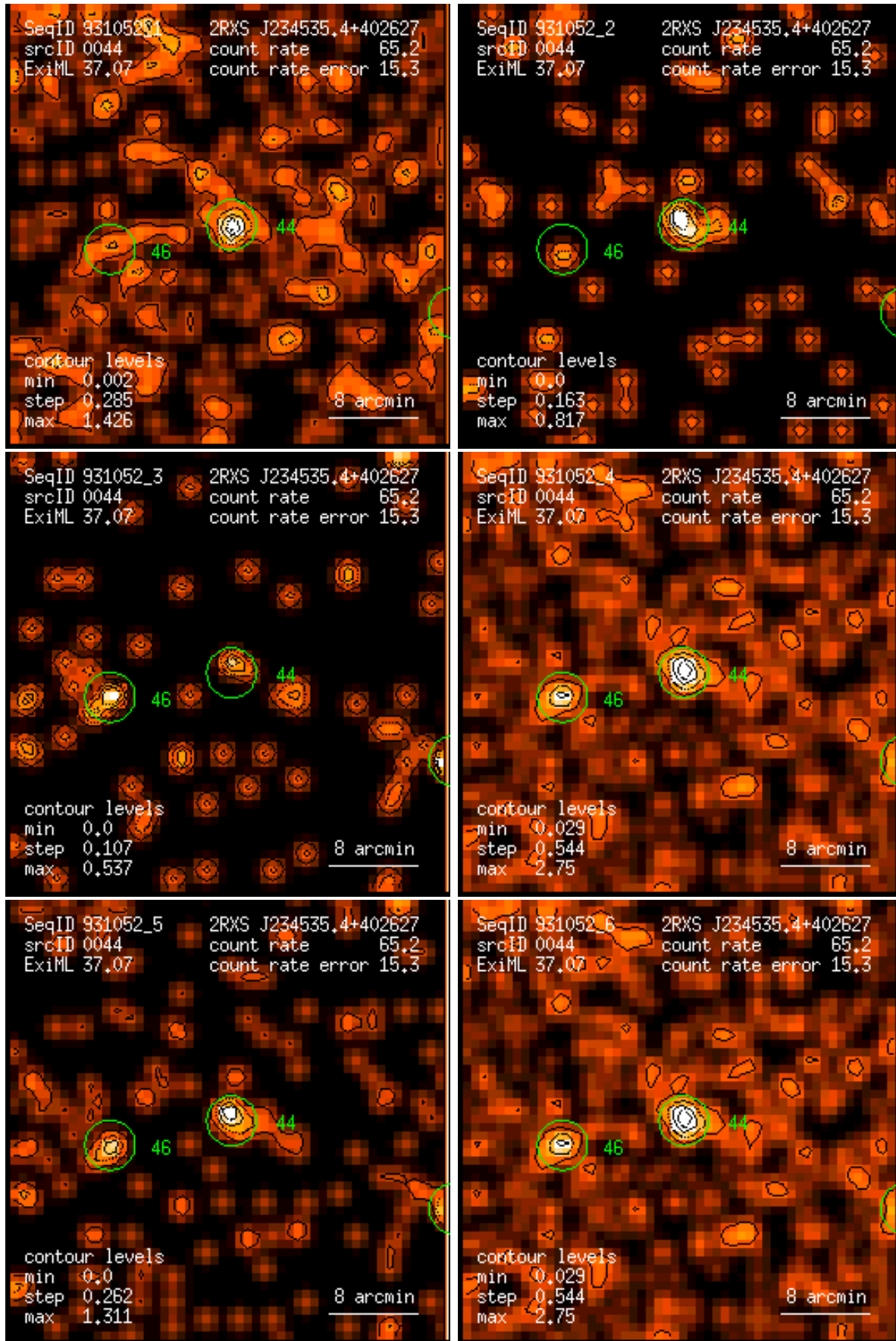
Figure 44: RASS 931052: detection 0044: band rate images, Gaussian filter: (1) PSPC channels 11 – 41, (2) 52 – 90, (3) 91 – 201, (4) 11 – 235, (5) 52 – 201, (6) 11 – 201. Broad band rates in counts/ks. Band rate contour levels in counts/ks/arcmin 2 .
