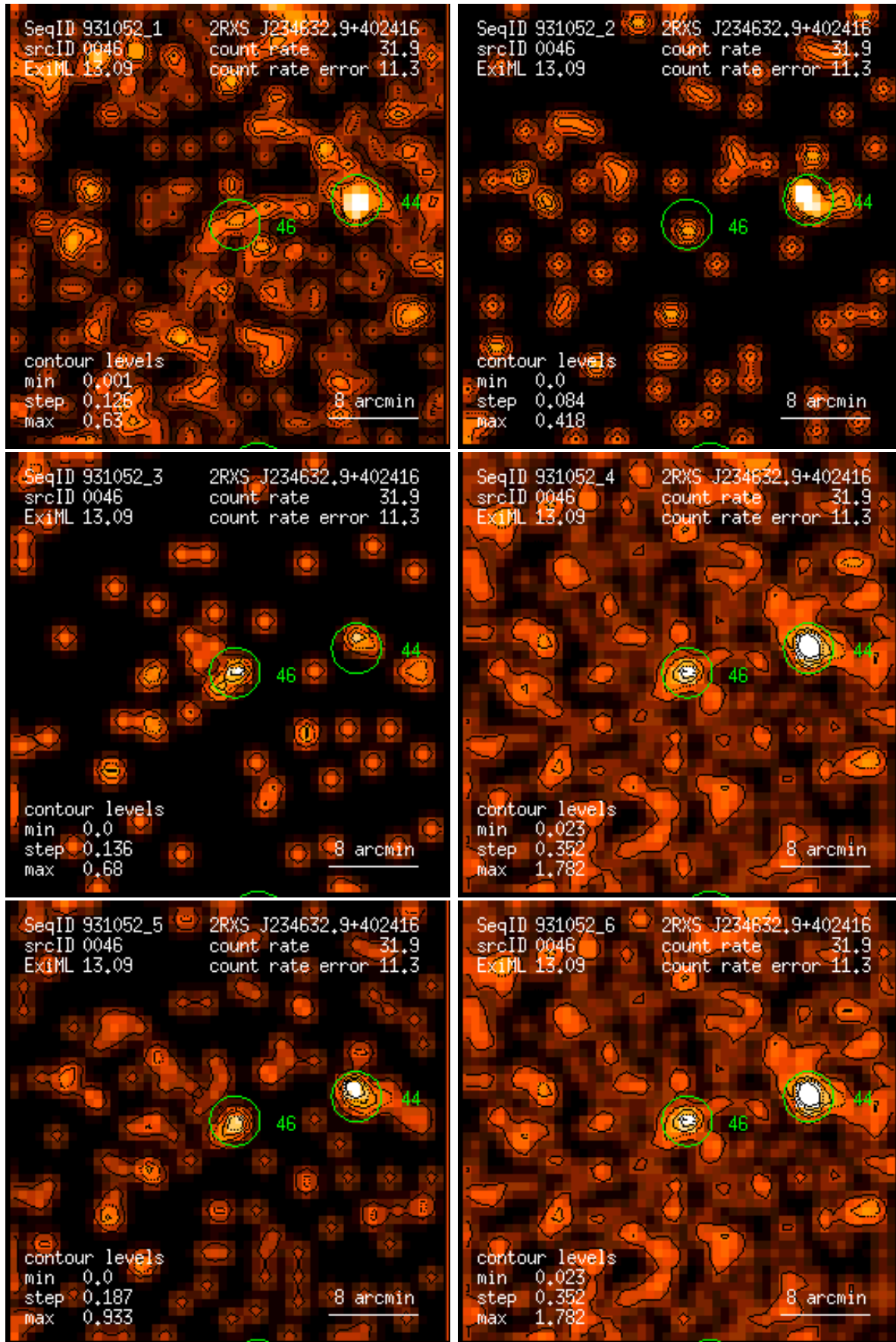
Figure 46: RASS 931052: detection 0046: band rate images, Gaussian filter: (1) PSPC channels 11 – 41, (2) 52 – 90, (3) 91 – 201, (4) 11 – 235, (5) 52 – 201, (6) 11 – 201. Broad band rates in counts/ks. Band rate contour levels in counts/ks/arcmin 2 .
