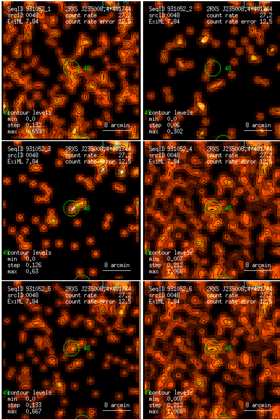
Figure 48: RASS 931052: detection 0048: band rate images, Gaussian filter: (1) PSPC channels 11 – 41, (2) 52 – 90, (3) 91 – 201, (4) 11 – 235, (5) 52 – 201, (6) 11 – 201. Broad band rates in counts/ks. Band rate contour levels in counts/ks/arcmin 2 .
