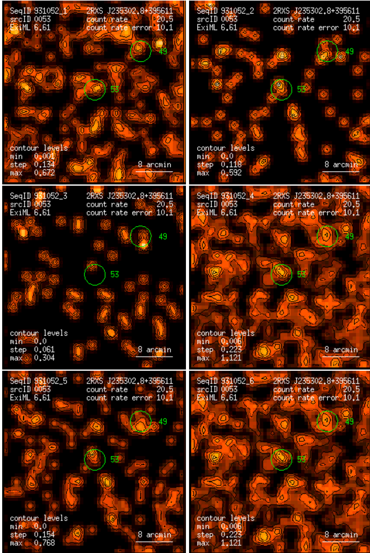
Figure 53: RASS 931052: detection 0053: band rate images, Gaussian filter: (1) PSPC channels 11 – 41, (2) 52 – 90, (3) 91 – 201, (4) 11 – 235, (5) 52 – 201, (6) 11 – 201. Broad band rates in counts/ks. Band rate contour levels in counts/ks/arcmin 2 .
