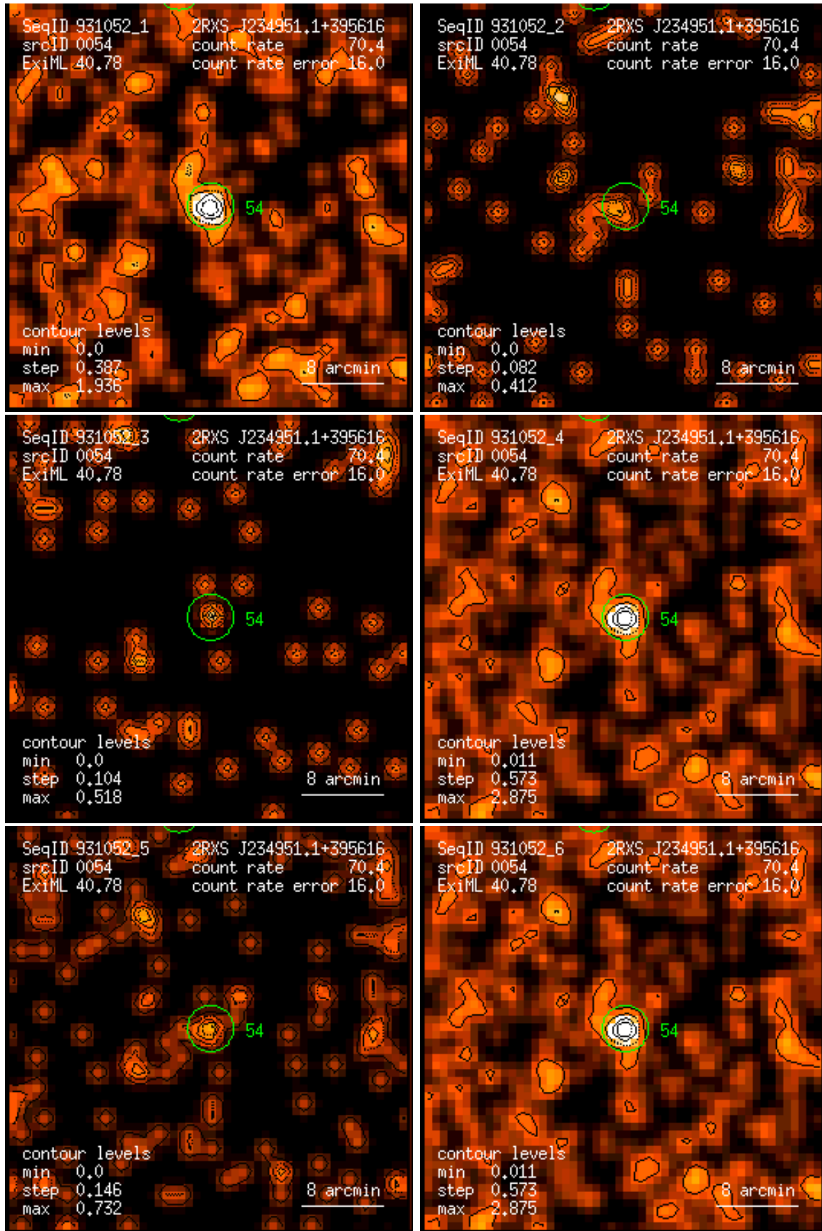
Figure 54: RASS 931052: detection 0054: band rate images, Gaussian filter: (1) PSPC channels 11 – 41, (2) 52 – 90, (3) 91 – 201, (4) 11 – 235, (5) 52 – 201, (6) 11 – 201. Broad band rates in counts/ks. Band rate contour levels in counts/ks/arcmin 2 .
