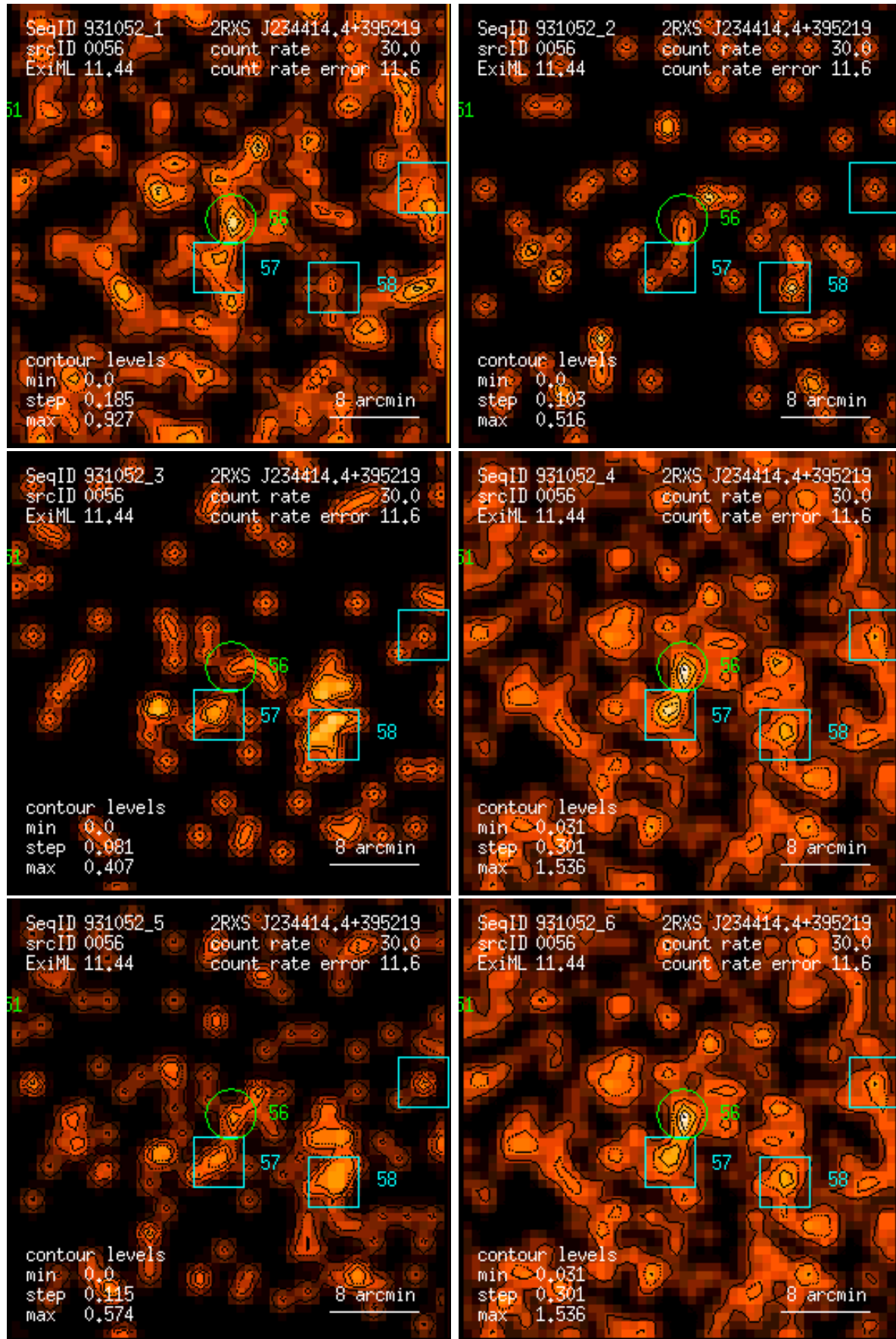
Figure 56: RASS 931052: detection 0056: band rate images, Gaussian filter: (1) PSPC channels 11 – 41, (2) 52 – 90, (3) 91 – 201, (4) 11 – 235, (5) 52 – 201, (6) 11 – 201. Broad band rates in counts/ks. Band rate contour levels in counts/ks/arcmin 2 .
