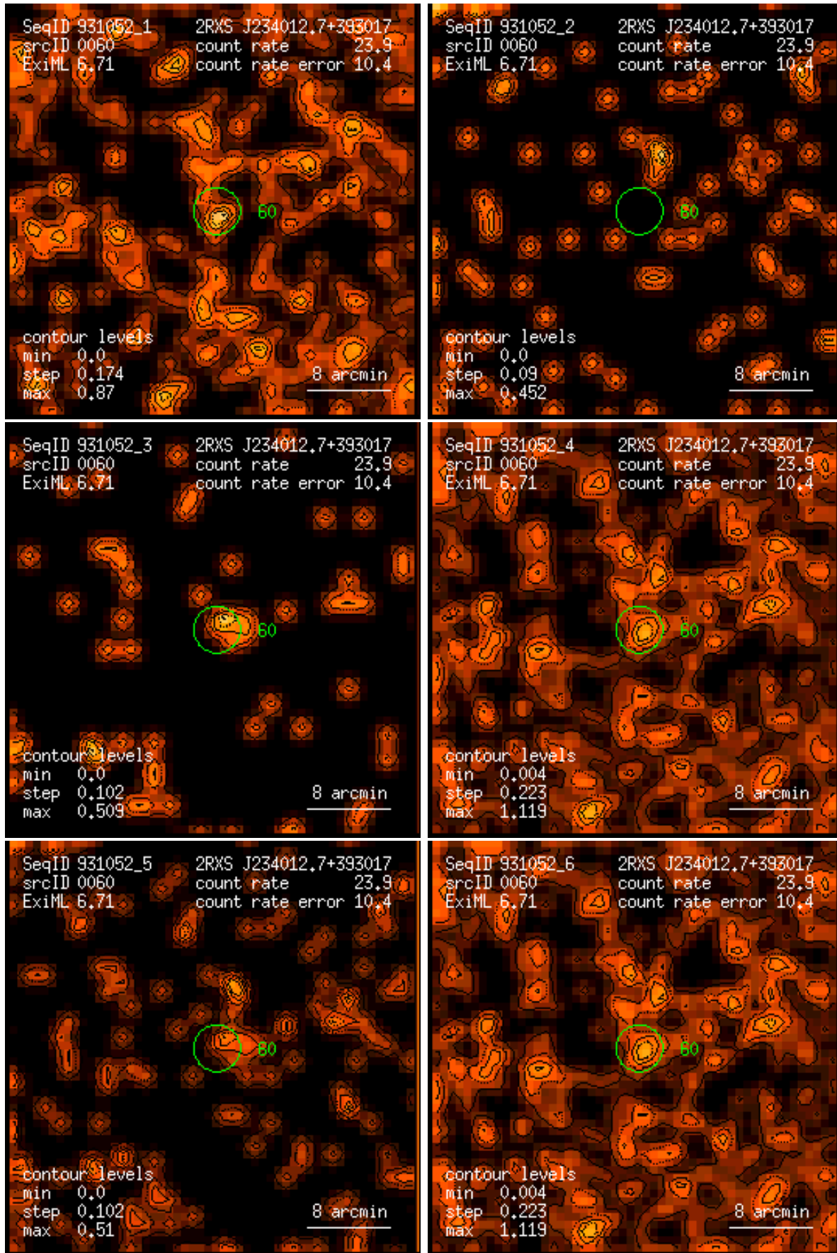
Figure 60: RASS 931052: detection 0060: band rate images, Gaussian filter: (1) PSPC channels 11 – 41, (2) 52 – 90, (3) 91 – 201, (4) 11 – 235, (5) 52 – 201, (6) 11 – 201. Broad band rates in counts/ks. Band rate contour levels in counts/ks/arcmin 2 .
