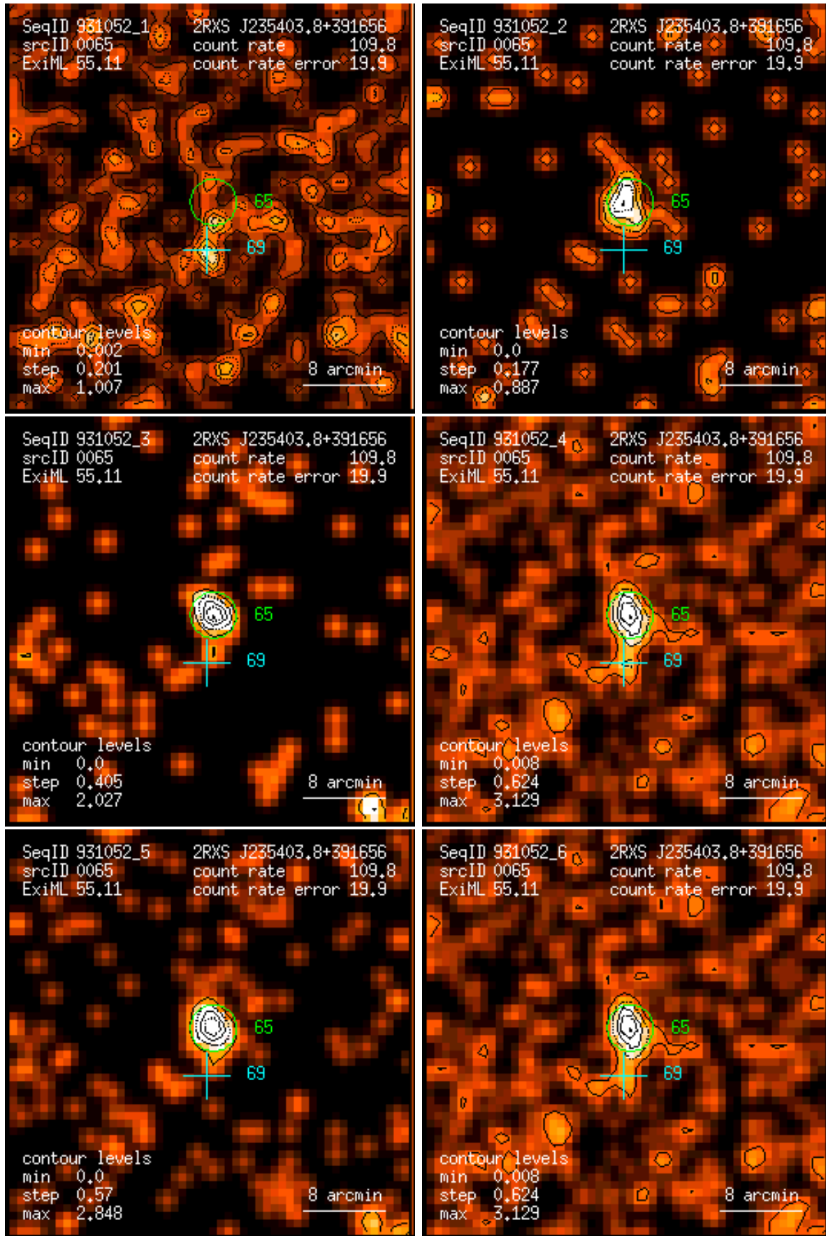
Figure 65: RASS 931052: detection 0065: band rate images, Gaussian filter: (1) PSPC channels 11 – 41, (2) 52 – 90, (3) 91 – 201, (4) 11 – 235, (5) 52 – 201, (6) 11 – 201. Broad band rates in counts/ks. Band rate contour levels in counts/ks/arcmin 2 .
