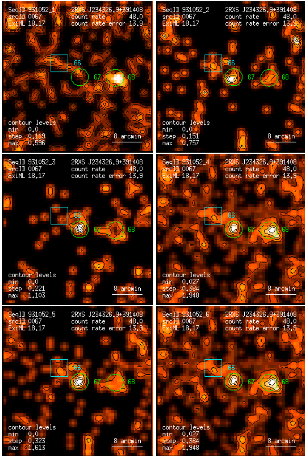
Figure 67: RASS 931052: detection 0067: band rate images, Gaussian filter: (1) PSPC channels 11 – 41, (2) 52 – 90, (3) 91 – 201, (4) 11 – 235, (5) 52 – 201, (6) 11 – 201. Broad band rates in counts/ks. Band rate contour levels in counts/ks/arcmin 2 .
