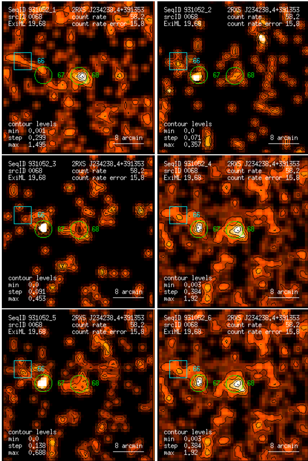
Figure 68: RASS 931052: detection 0068: band rate images, Gaussian filter: (1) PSPC channels 11 – 41, (2) 52 – 90, (3) 91 – 201, (4) 11 – 235, (5) 52 – 201, (6) 11 – 201. Broad band rates in counts/ks. Band rate contour levels in counts/ks/arcmin 2 .
