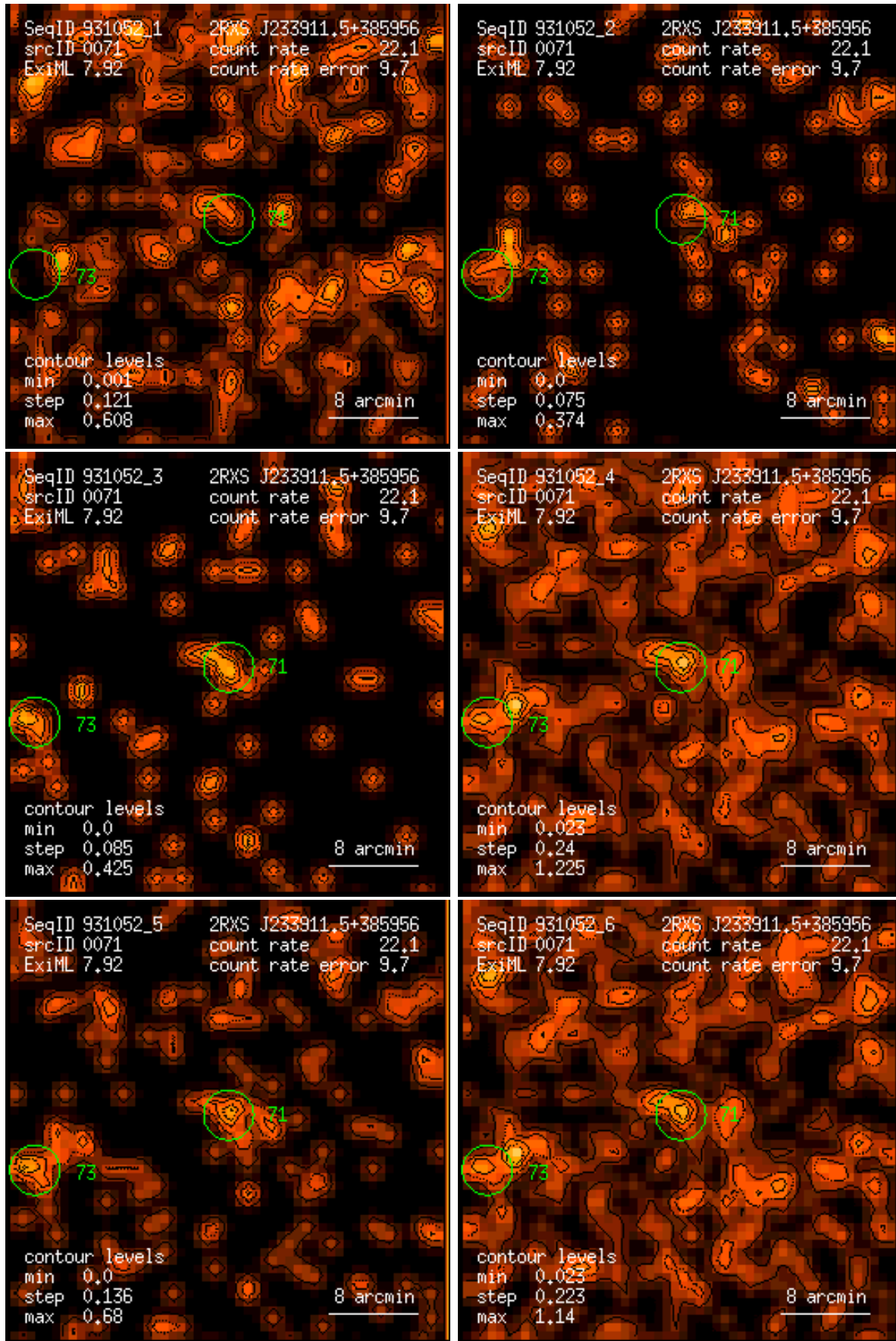
Figure 71: RASS 931052: detection 0071: band rate images, Gaussian filter: (1) PSPC channels 11 – 41, (2) 52 – 90, (3) 91 – 201, (4) 11 – 235, (5) 52 – 201, (6) 11 – 201. Broad band rates in counts/ks. Band rate contour levels in counts/ks/arcmin 2 .
