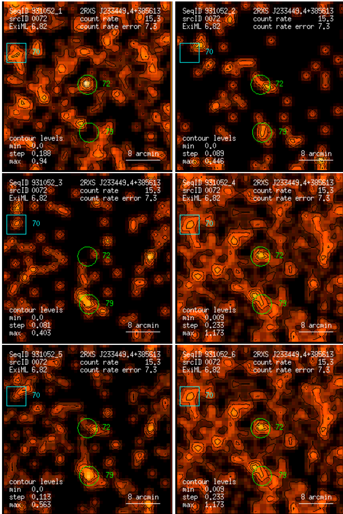
Figure 72: RASS 931052: detection 0072: band rate images, Gaussian filter: (1) PSPC channels 11 – 41, (2) 52 – 90, (3) 91 – 201, (4) 11 – 235, (5) 52 – 201, (6) 11 – 201. Broad band rates in counts/ks. Band rate contour levels in counts/ks/arcmin 2 .
