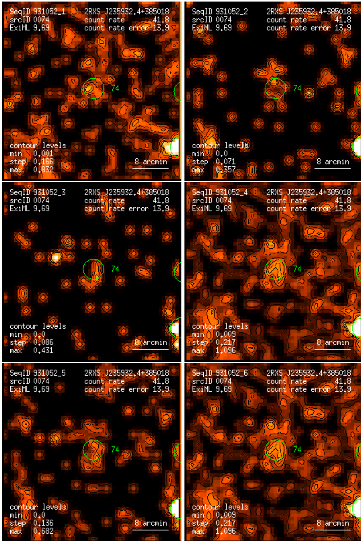
Figure 74: RASS 931052: detection 0074: band rate images, Gaussian filter: (1) PSPC channels 11 – 41, (2) 52 – 90, (3) 91 – 201, (4) 11 – 235, (5) 52 – 201, (6) 11 – 201. Broad band rates in counts/ks. Band rate contour levels in counts/ks/arcmin 2 .
