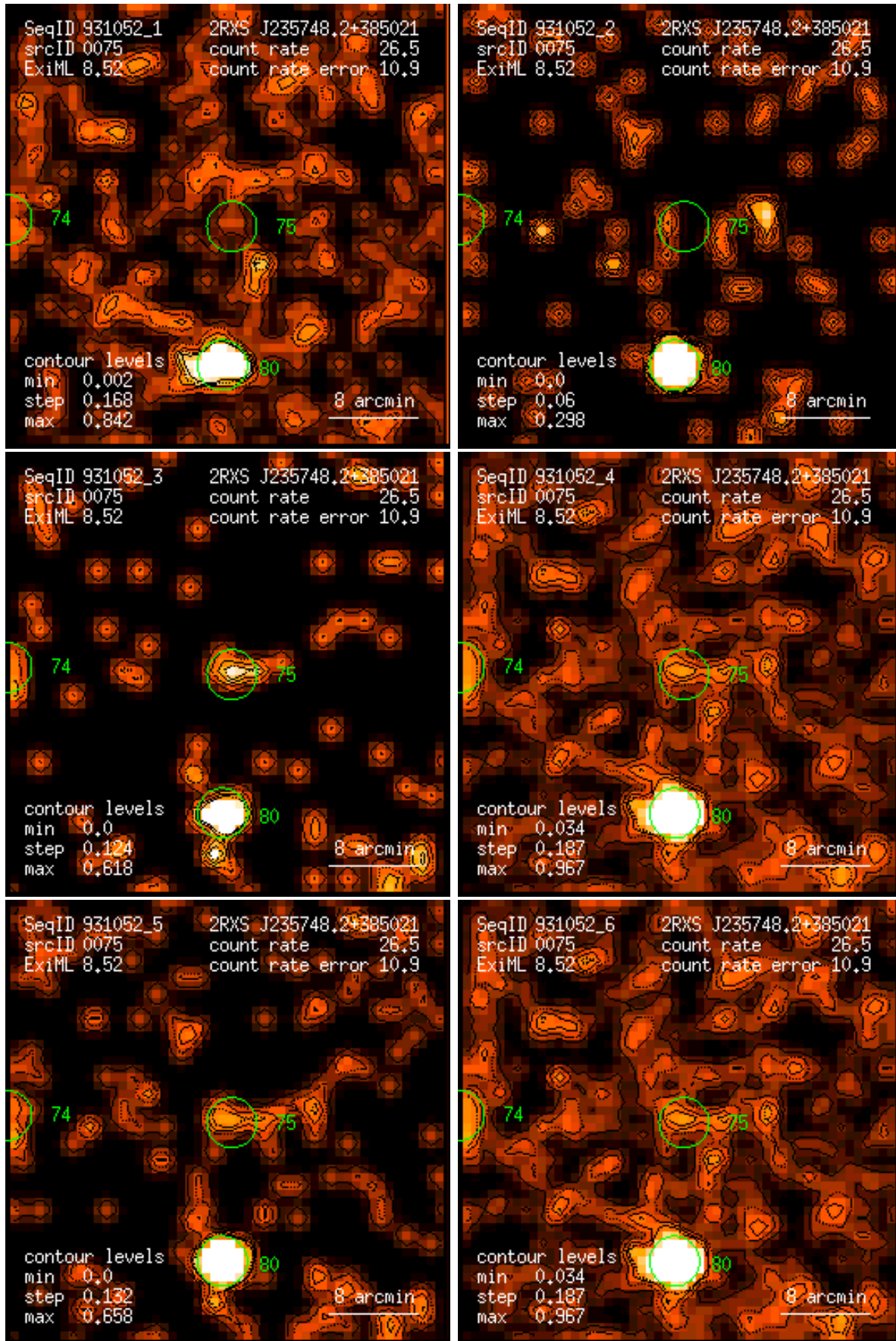
Figure 75: RASS 931052: detection 0075: band rate images, Gaussian filter: (1) PSPC channels 11 – 41, (2) 52 – 90, (3) 91 – 201, (4) 11 – 235, (5) 52 – 201, (6) 11 – 201. Broad band rates in counts/ks. Band rate contour levels in counts/ks/arcmin 2 .
