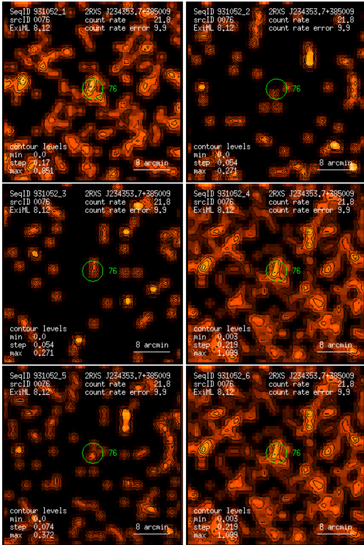
Figure 76: RASS 931052: detection 0076: band rate images, Gaussian filter: (1) PSPC channels 11 – 41, (2) 52 – 90, (3) 91 – 201, (4) 11 – 235, (5) 52 – 201, (6) 11 – 201. Broad band rates in counts/ks. Band rate contour levels in counts/ks/arcmin 2 .
