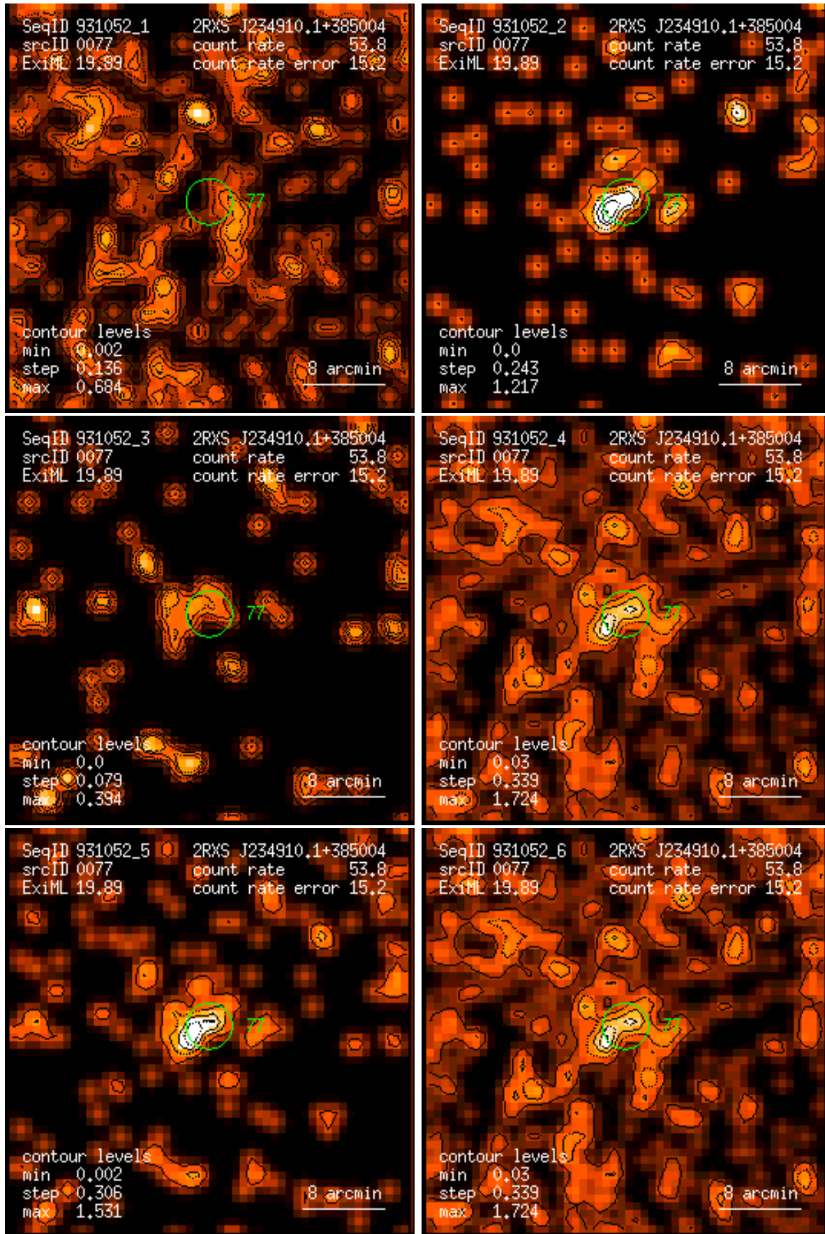
Figure 77: RASS 931052: detection 0077: band rate images, Gaussian filter: (1) PSPC channels 11 – 41, (2) 52 – 90, (3) 91 – 201, (4) 11 – 235, (5) 52 – 201, (6) 11 – 201. Broad band rates in counts/ks. Band rate contour levels in counts/ks/arcmin 2 .
