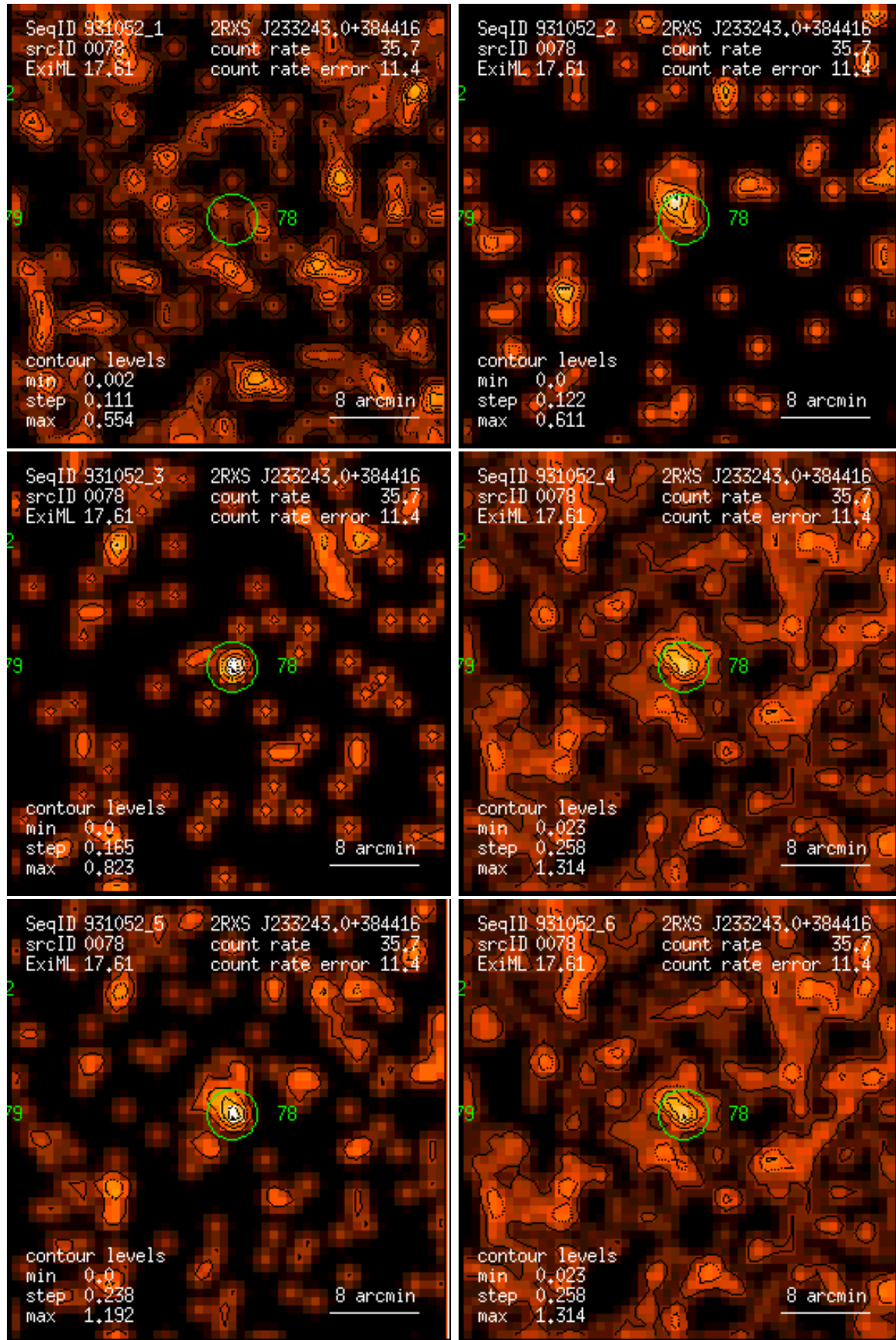
Figure 78: RASS 931052: detection 0078: band rate images, Gaussian filter: (1) PSPC channels 11 – 41, (2) 52 – 90, (3) 91 – 201, (4) 11 – 235, (5) 52 – 201, (6) 11 – 201. Broad band rates in counts/ks. Band rate contour levels in counts/ks/arcmin 2 .
