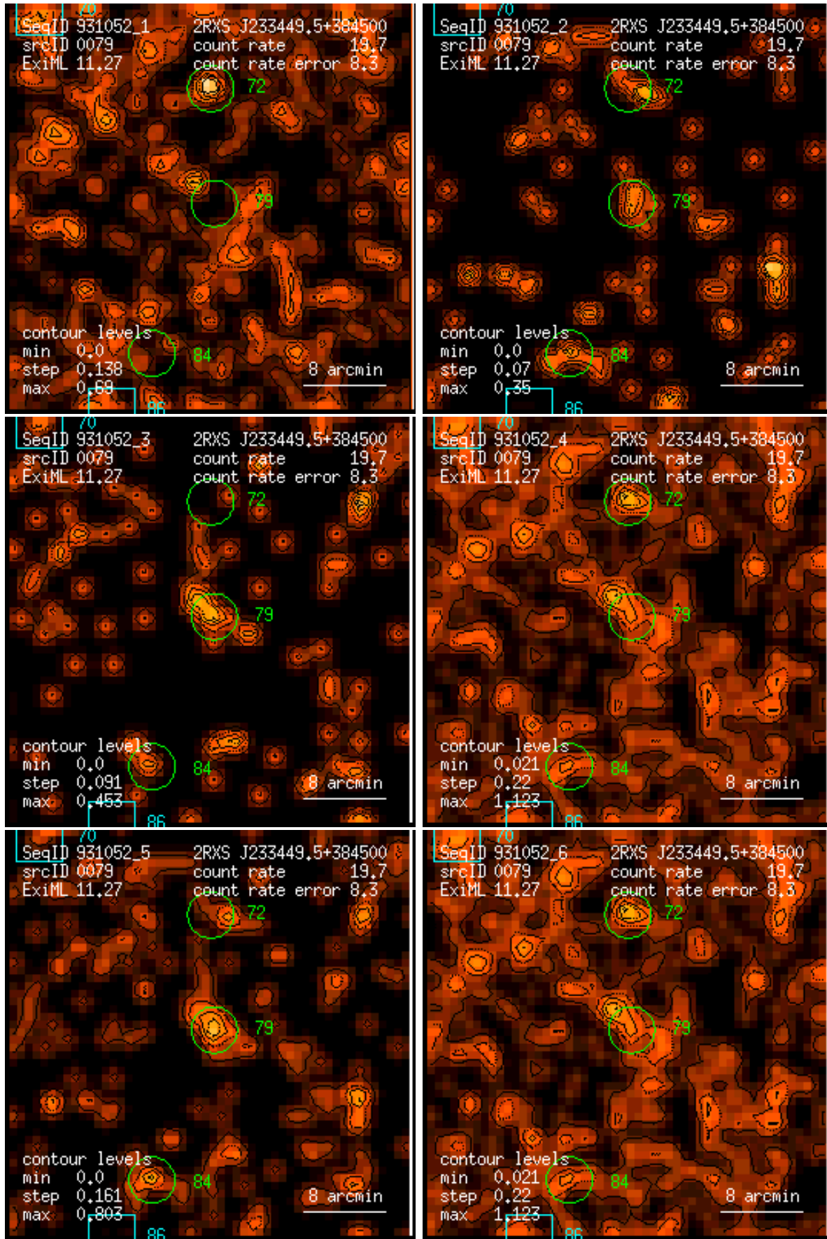
Figure 79: RASS 931052: detection 0079: band rate images, Gaussian filter: (1) PSPC channels 11 – 41, (2) 52 – 90, (3) 91 – 201, (4) 11 – 235, (5) 52 – 201, (6) 11 – 201. Broad band rates in counts/ks. Band rate contour levels in counts/ks/arcmin 2 .
