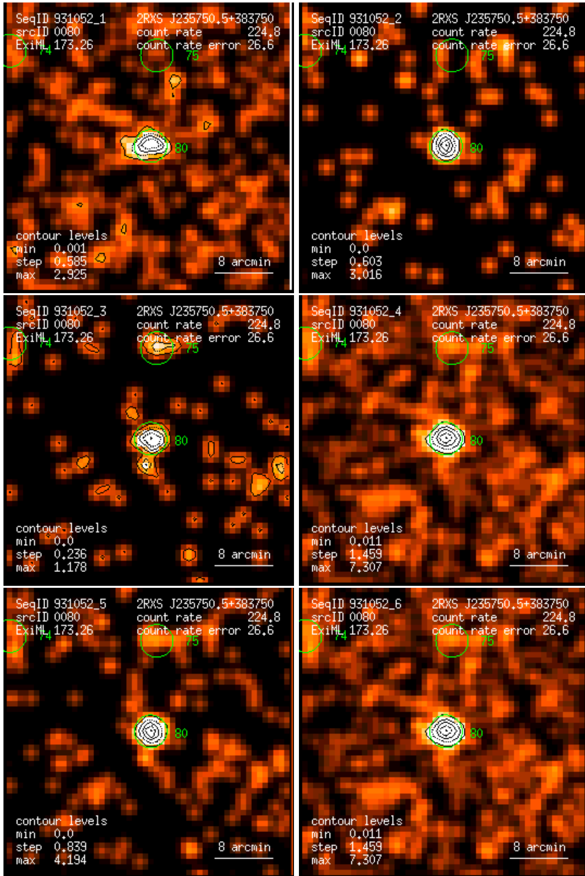
Figure 80: RASS 931052: detection 0080: band rate images, Gaussian filter: (1) PSPC channels 11 – 41, (2) 52 – 90, (3) 91 – 201, (4) 11 – 235, (5) 52 – 201, (6) 11 – 201. Broad band rates in counts/ks. Band rate contour levels in counts/ks/arcmin 2 .
