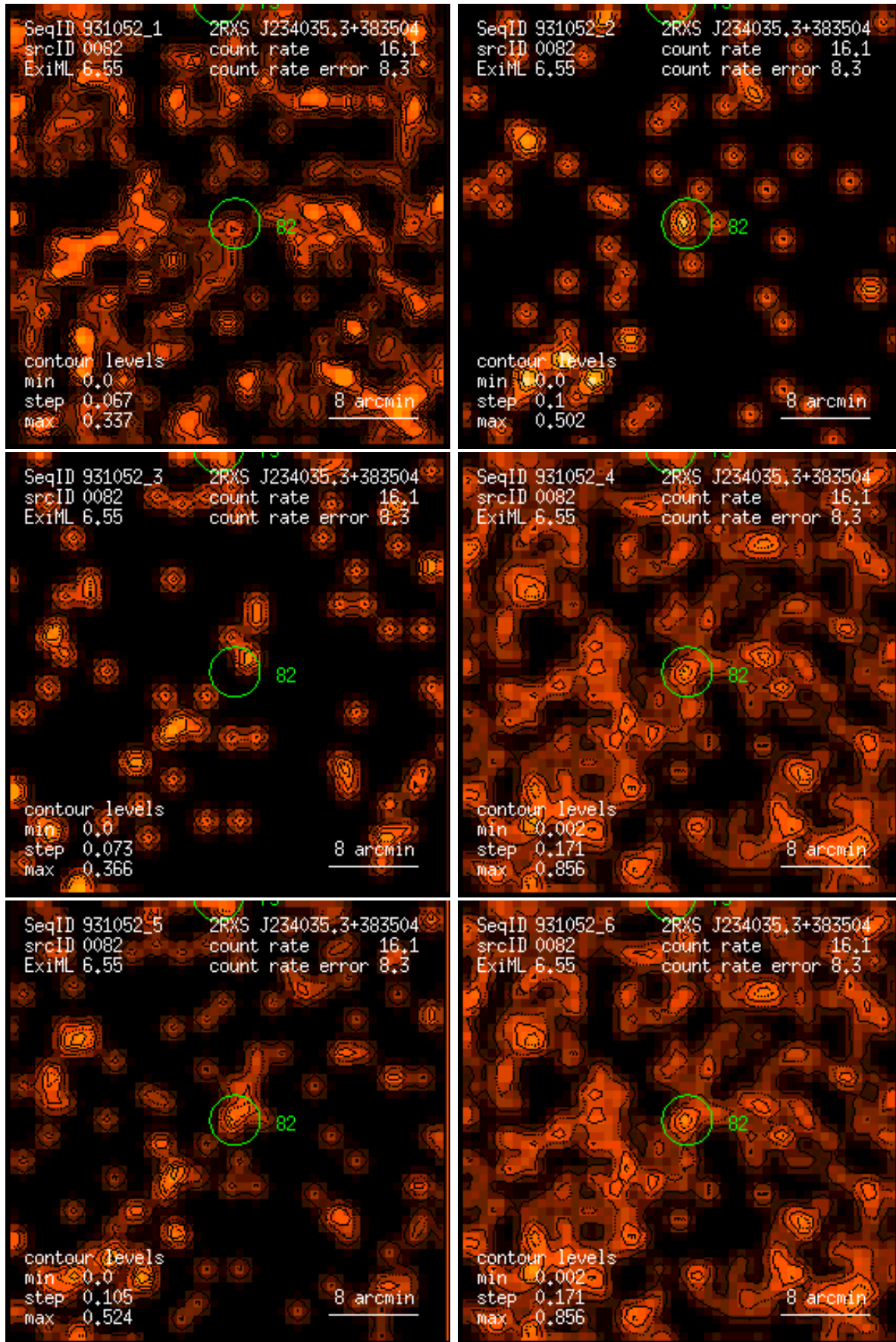
Figure 82: RASS 931052: detection 0082: band rate images, Gaussian filter: (1) PSPC channels 11 – 41, (2) 52 – 90, (3) 91 – 201, (4) 11 – 235, (5) 52 – 201, (6) 11 – 201. Broad band rates in counts/ks. Band rate contour levels in counts/ks/arcmin 2 .
