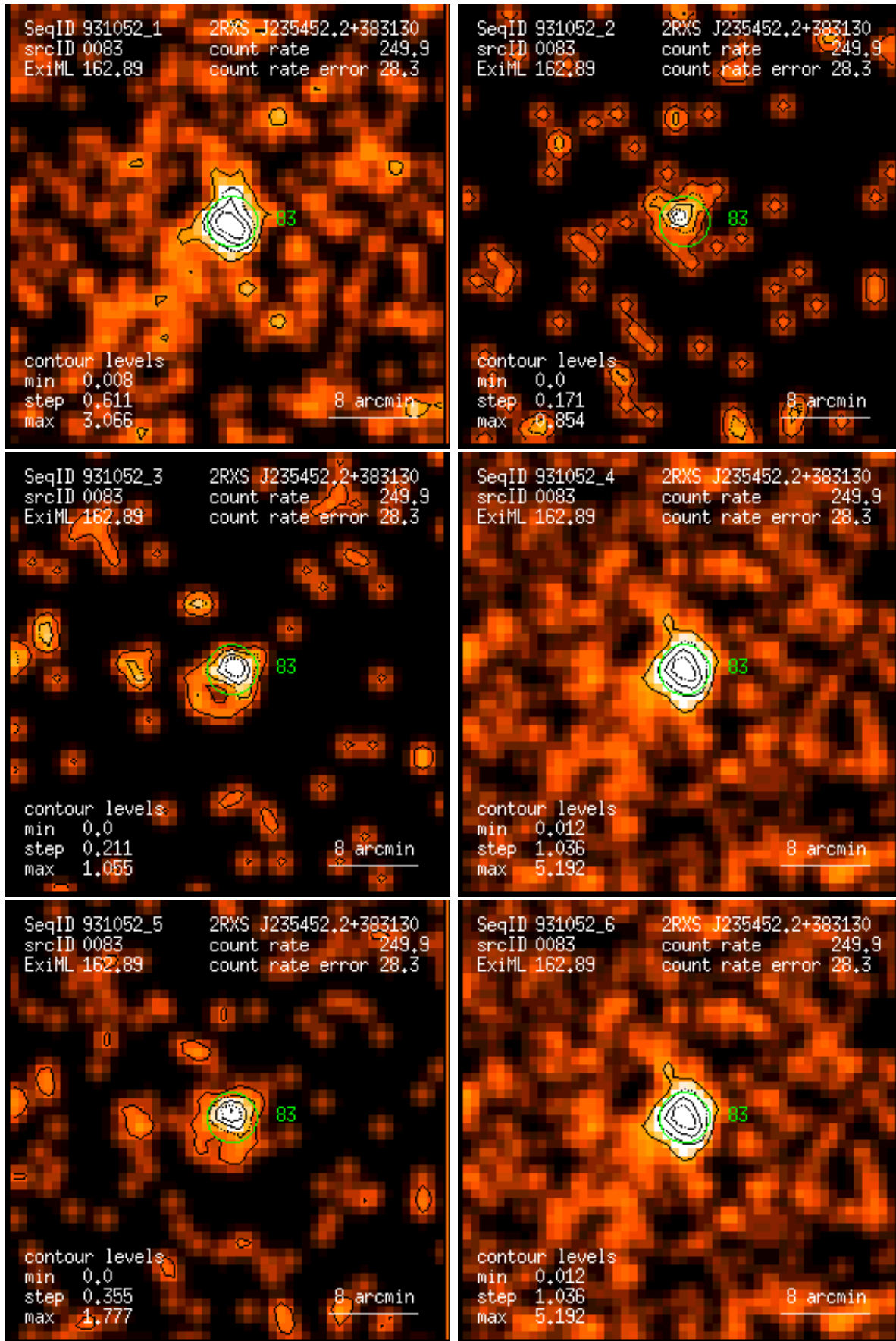
Figure 83: RASS 931052: detection 0083: band rate images, Gaussian filter: (1) PSPC channels 11 – 41, (2) 52 – 90, (3) 91 – 201, (4) 11 – 235, (5) 52 – 201, (6) 11 – 201. Broad band rates in counts/ks. Band rate contour levels in counts/ks/arcmin 2 .
