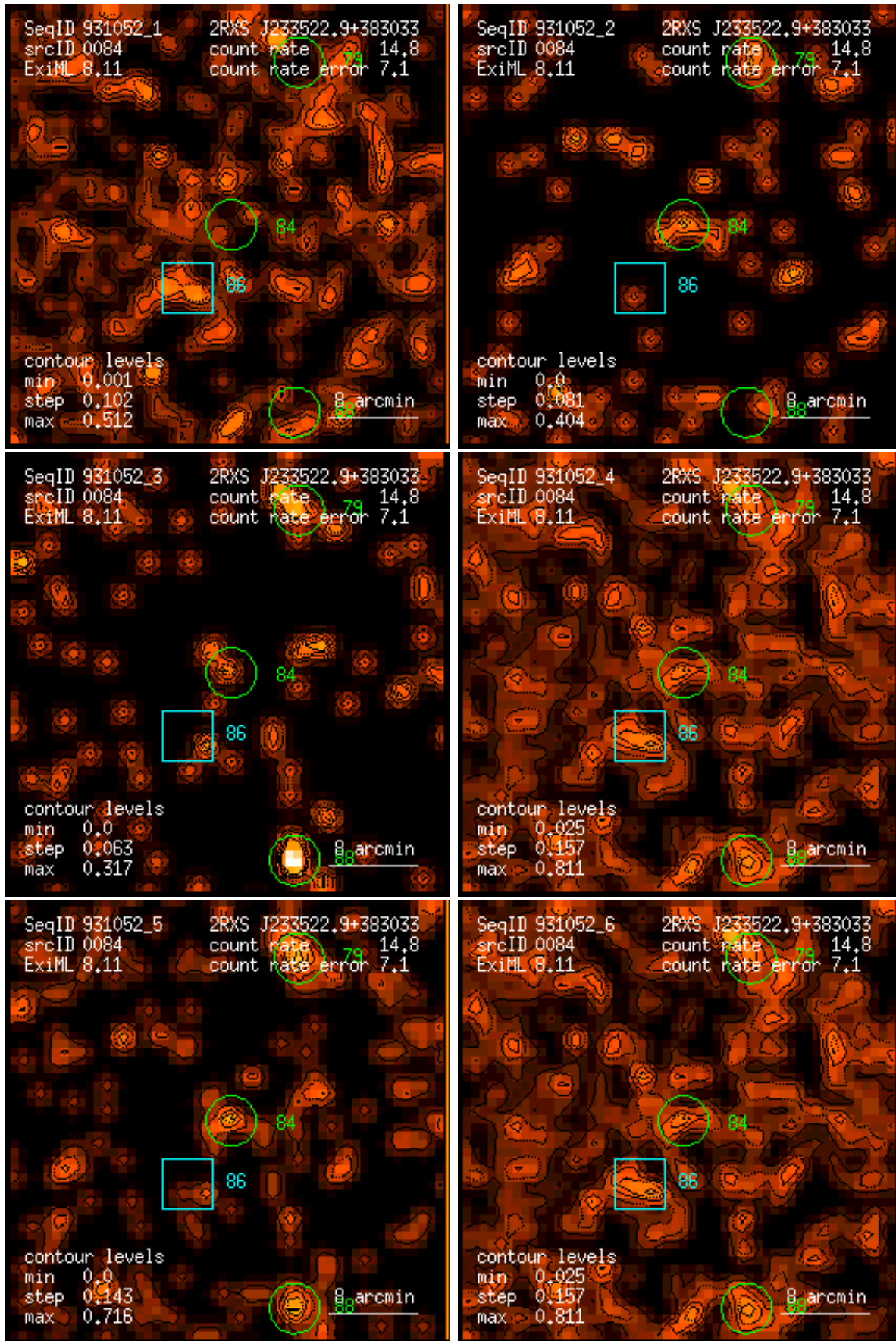
Figure 84: RASS 931052: detection 0084: band rate images, Gaussian filter: (1) PSPC channels 11 – 41, (2) 52 – 90, (3) 91 – 201, (4) 11 – 235, (5) 52 – 201, (6) 11 – 201. Broad band rates in counts/ks. Band rate contour levels in counts/ks/arcmin 2 .
