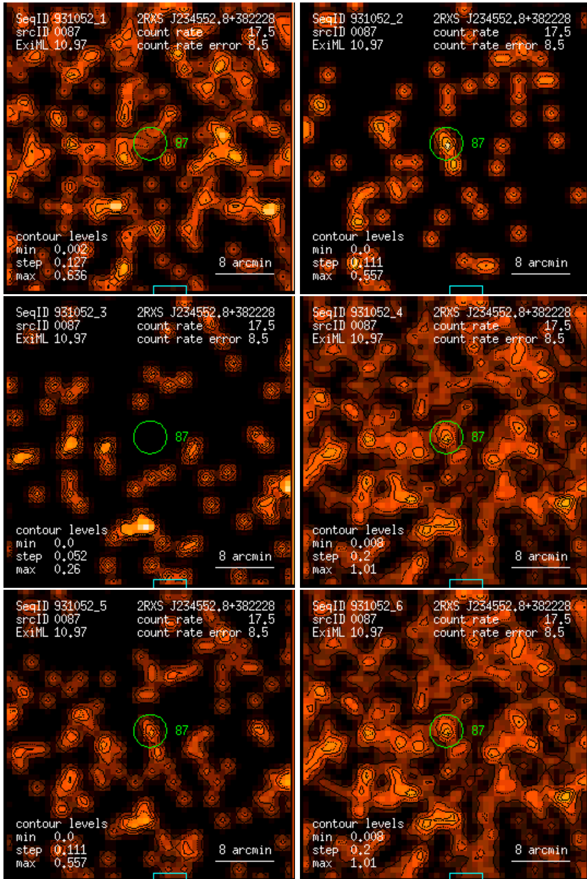
Figure 87: RASS 931052: detection 0087: band rate images, Gaussian filter: (1) PSPC channels 11 – 41, (2) 52 – 90, (3) 91 – 201, (4) 11 – 235, (5) 52 – 201, (6) 11 – 201. Broad band rates in counts/ks. Band rate contour levels in counts/ks/arcmin 2 .
