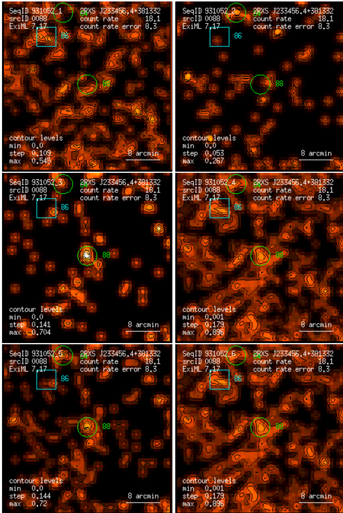
Figure 88: RASS 931052: detection 0088: band rate images, Gaussian filter: (1) PSPC channels 11 – 41, (2) 52 – 90, (3) 91 – 201, (4) 11 – 235, (5) 52 – 201, (6) 11 – 201. Broad band rates in counts/ks. Band rate contour levels in counts/ks/arcmin 2 .
