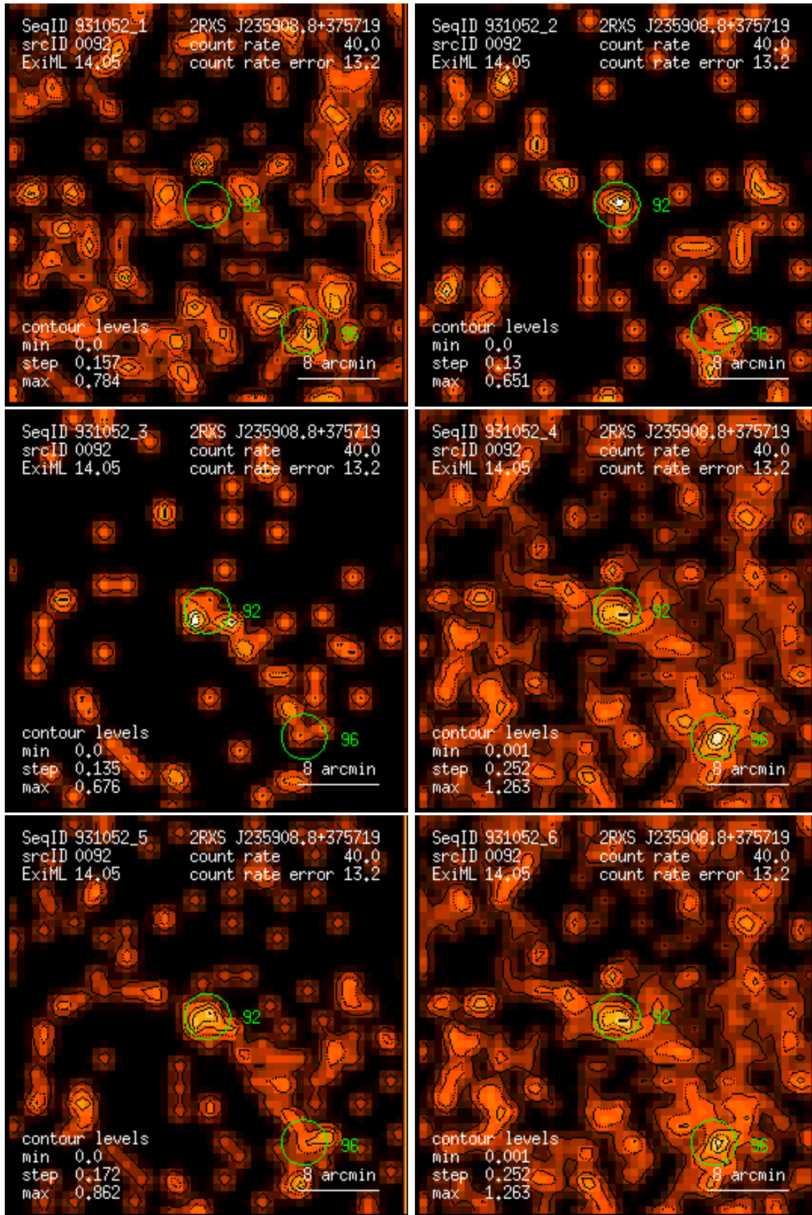
Figure 92: RASS 931052: detection 0092: band rate images, Gaussian filter: (1) PSPC channels 11 – 41, (2) 52 – 90, (3) 91 – 201, (4) 11 – 235, (5) 52 – 201, (6) 11 – 201. Broad band rates in counts/ks. Band rate contour levels in counts/ks/arcmin 2 .
