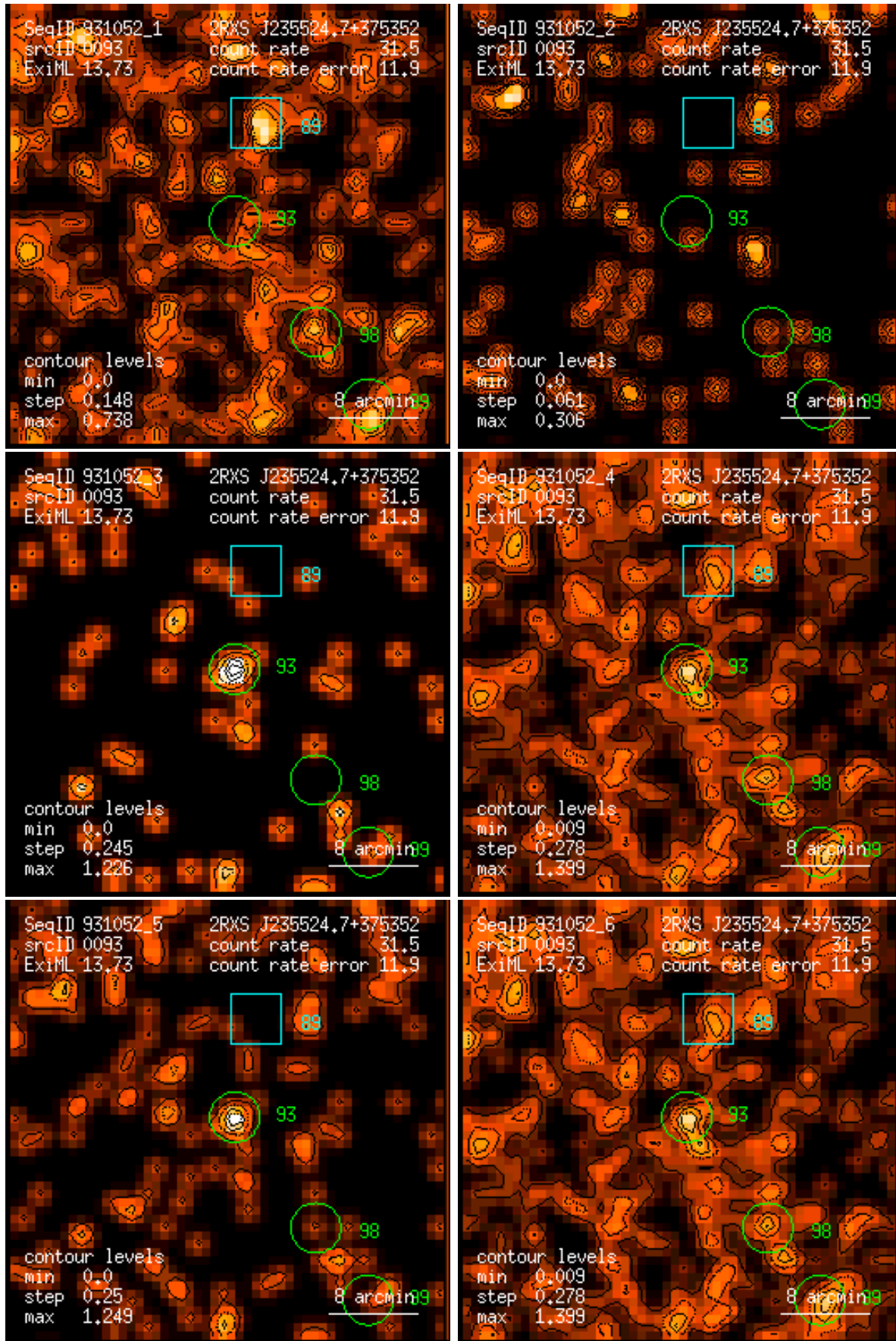
Figure 93: RASS 931052: detection 0093: band rate images, Gaussian filter: (1) PSPC channels 11 – 41, (2) 52 – 90, (3) 91 – 201, (4) 11 – 235, (5) 52 – 201, (6) 11 – 201. Broad band rates in counts/ks. Band rate contour levels in counts/ks/arcmin 2 .
