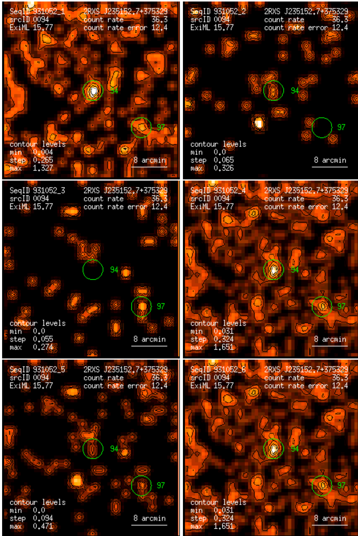
Figure 94: RASS 931052: detection 0094: band rate images, Gaussian filter: (1) PSPC channels 11 – 41, (2) 52 – 90, (3) 91 – 201, (4) 11 – 235, (5) 52 – 201, (6) 11 – 201. Broad band rates in counts/ks. Band rate contour levels in counts/ks/arcmin 2 .
