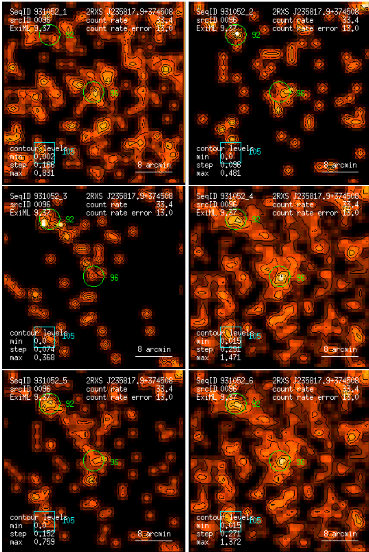
Figure 96: RASS 931052: detection 0096: band rate images, Gaussian filter: (1) PSPC channels 11 – 41, (2) 52 – 90, (3) 91 – 201, (4) 11 – 235, (5) 52 – 201, (6) 11 – 201. Broad band rates in counts/ks. Band rate contour levels in counts/ks/arcmin 2 .
