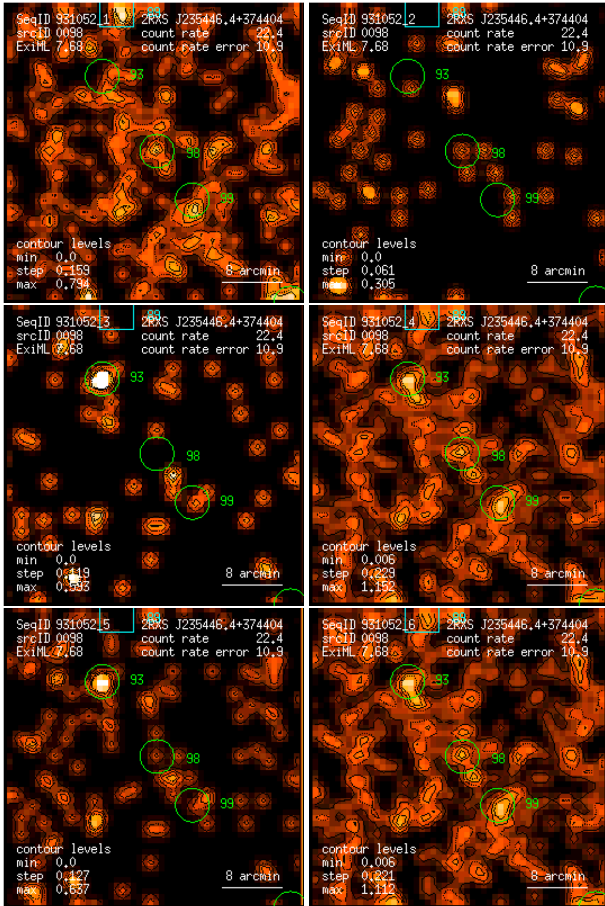
Figure 98: RASS 931052: detection 0098: band rate images, Gaussian filter: (1) PSPC channels 11 – 41, (2) 52 – 90, (3) 91 – 201, (4) 11 – 235, (5) 52 – 201, (6) 11 – 201. Broad band rates in counts/ks. Band rate contour levels in counts/ks/arcmin 2 .
