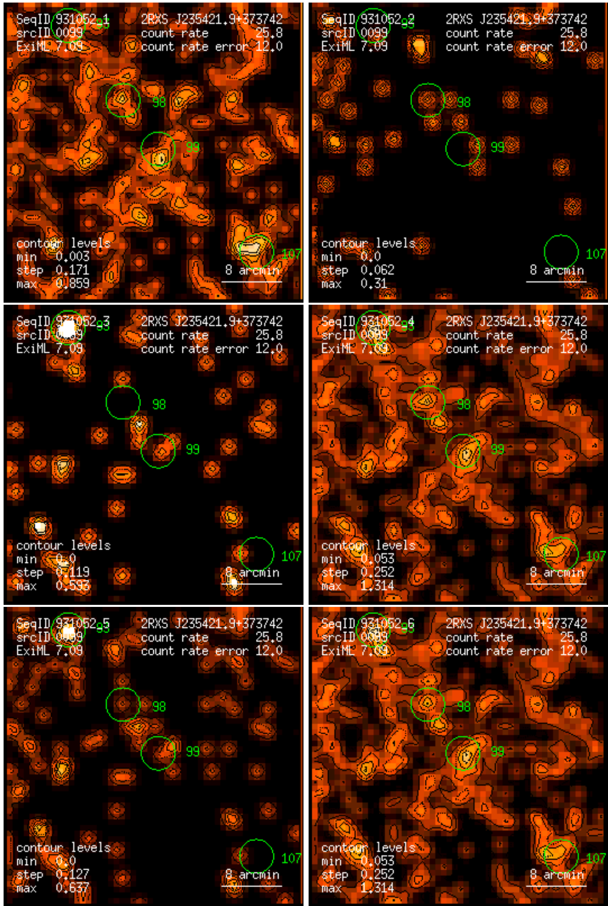
Figure 99: RASS 931052: detection 0099: band rate images, Gaussian filter: (1) PSPC channels 11 – 41, (2) 52 – 90, (3) 91 – 201, (4) 11 – 235, (5) 52 – 201, (6) 11 – 201. Broad band rates in counts/ks. Band rate contour levels in counts/ks/arcmin 2 .
