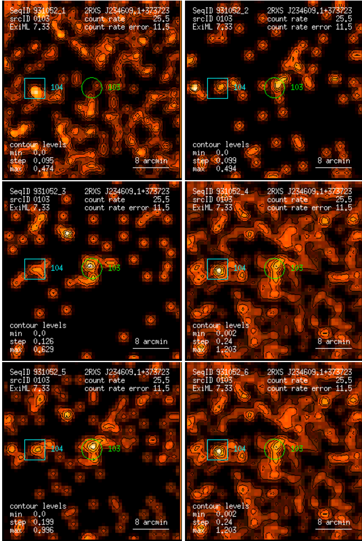
Figure 103: RASS 931052: detection 0103: band rate images, Gaussian filter: (1) PSPC channels 11 – 41, (2) 52 – 90, (3) 91 – 201, (4) 11 – 235, (5) 52 – 201, (6) 11 – 201. Broad band rates in counts/ks. Band rate contour levels in counts/ks/arcmin 2 .
