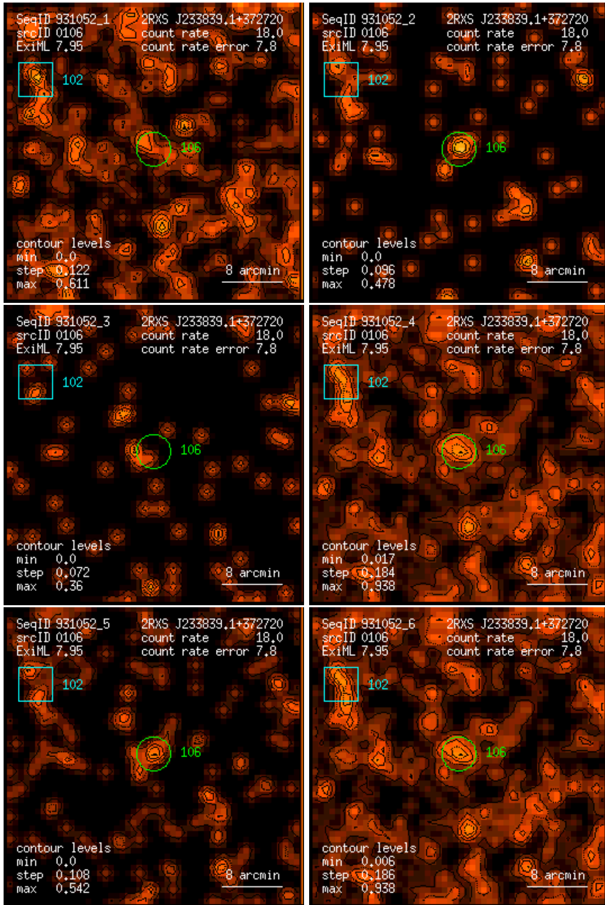
Figure 106: RASS 931052: detection 0106: band rate images, Gaussian filter: (1) PSPC channels 11 – 41, (2) 52 – 90, (3) 91 – 201, (4) 11 – 235, (5) 52 – 201, (6) 11 – 201. Broad band rates in counts/ks. Band rate contour levels in counts/ks/arcmin 2 .
