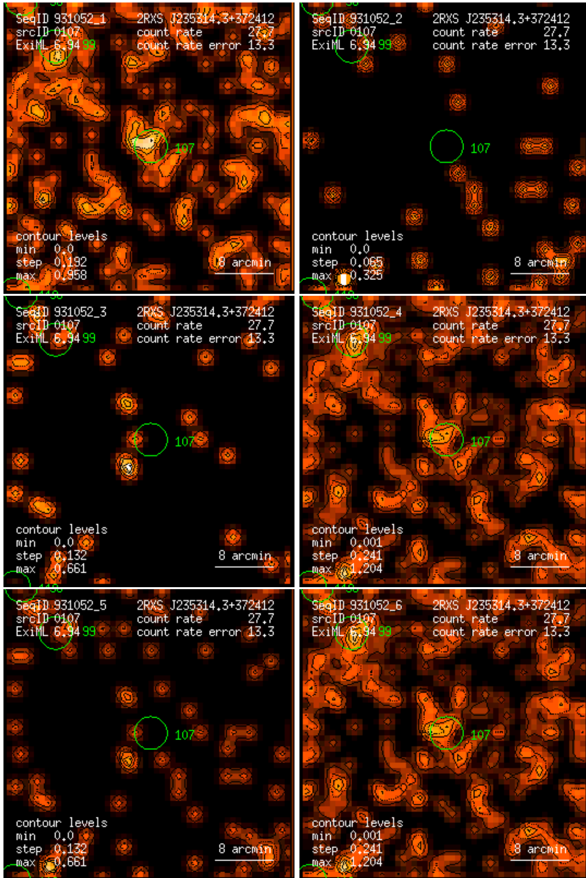
Figure 107: RASS 931052: detection 0107: band rate images, Gaussian filter: (1) PSPC channels 11 – 41, (2) 52 – 90, (3) 91 – 201, (4) 11 – 235, (5) 52 – 201, (6) 11 – 201. Broad band rates in counts/ks. Band rate contour levels in counts/ks/arcmin 2 .
