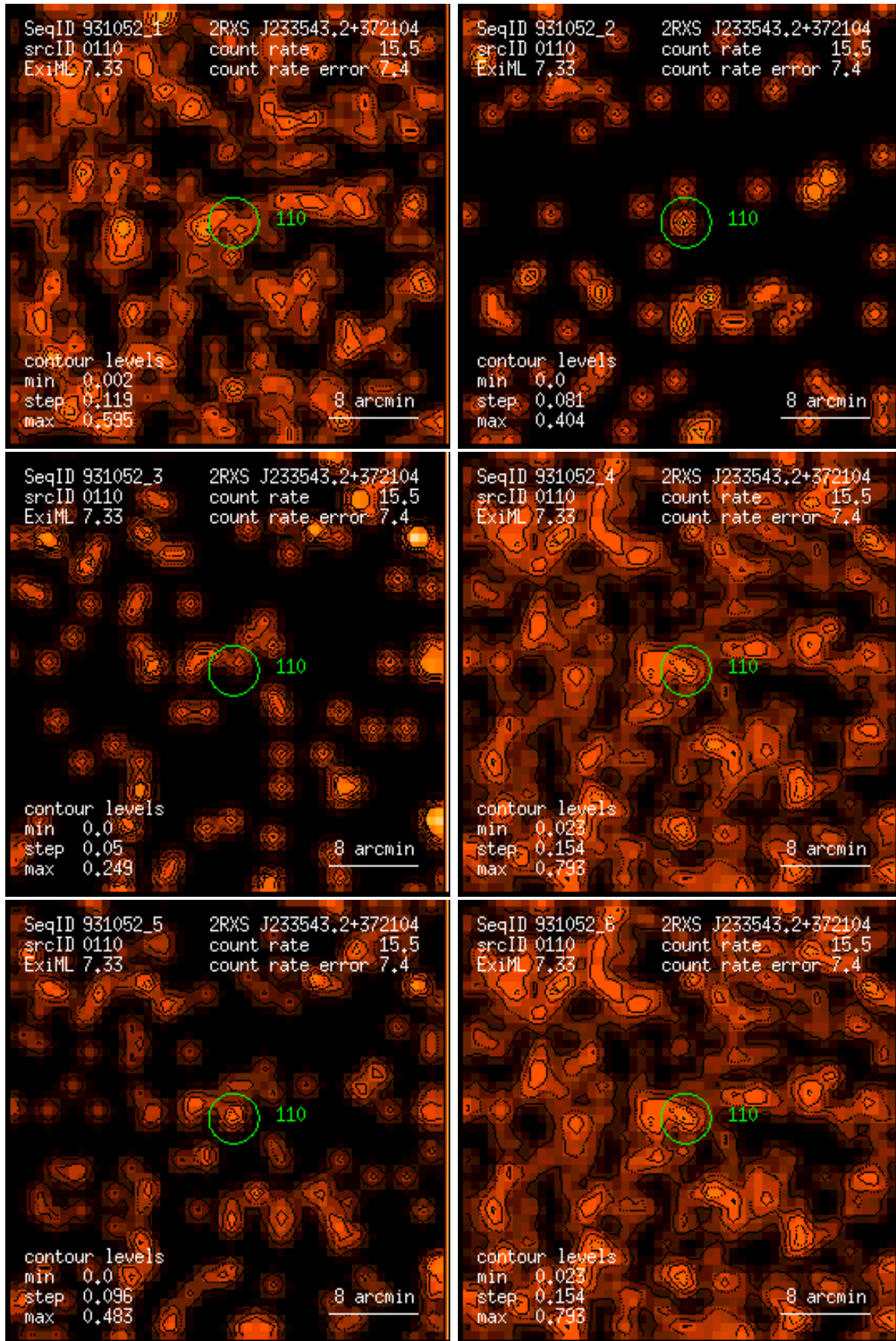
Figure 110: RASS 931052: detection 0110: band rate images, Gaussian filter: (1) PSPC channels 11 – 41, (2) 52 – 90, (3) 91 – 201, (4) 11 – 235, (5) 52 – 201, (6) 11 – 201. Broad band rates in counts/ks. Band rate contour levels in counts/ks/arcmin 2 .
